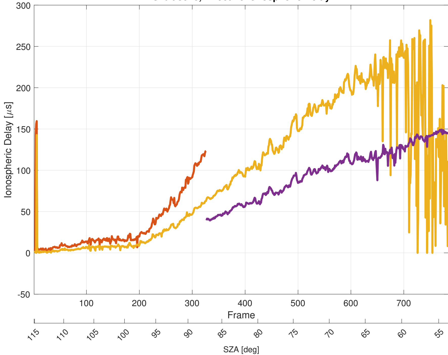
Orbit 9573, Effective Ionospheric Delay
