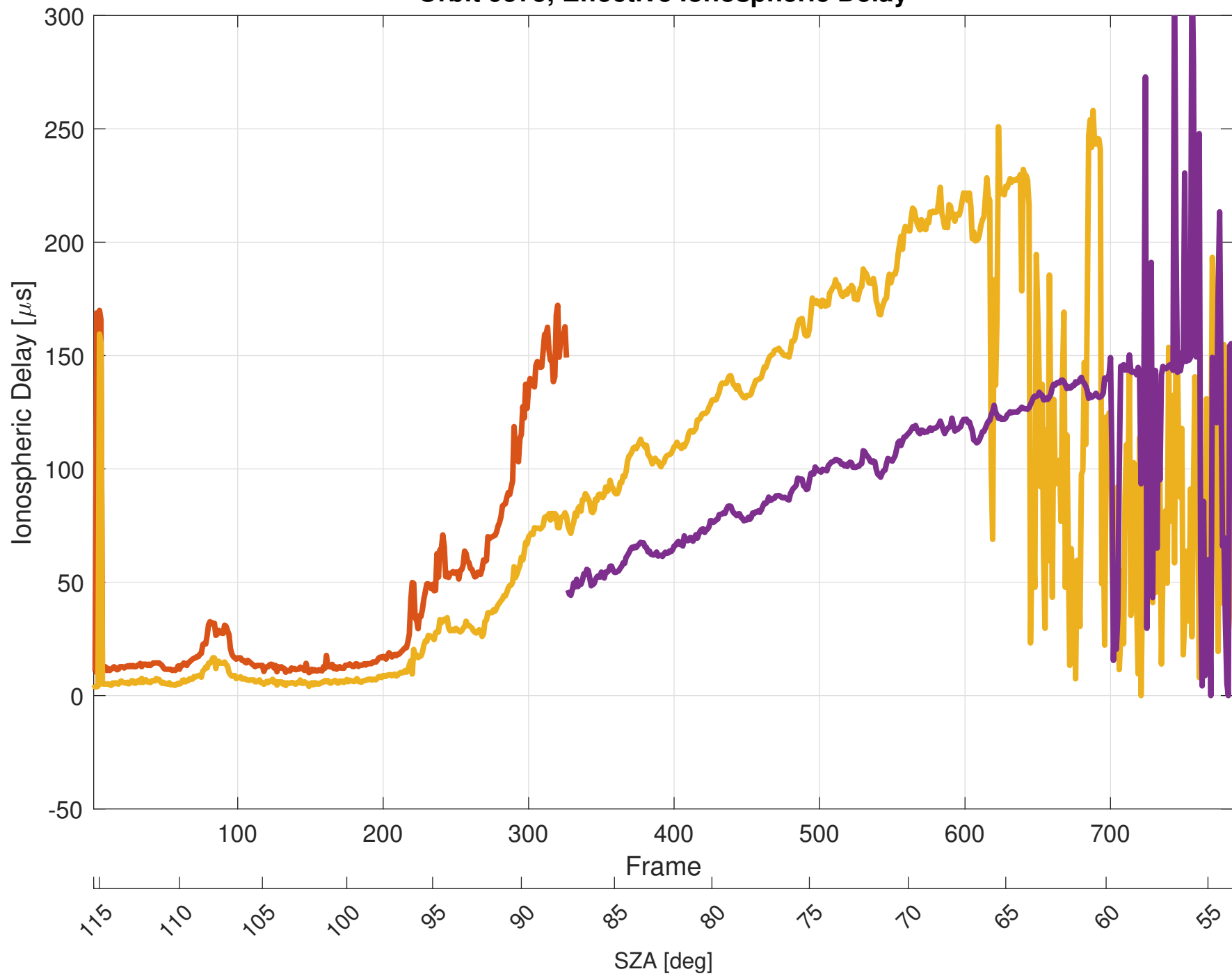
Orbit 9575, Effective Ionospheric Delay
