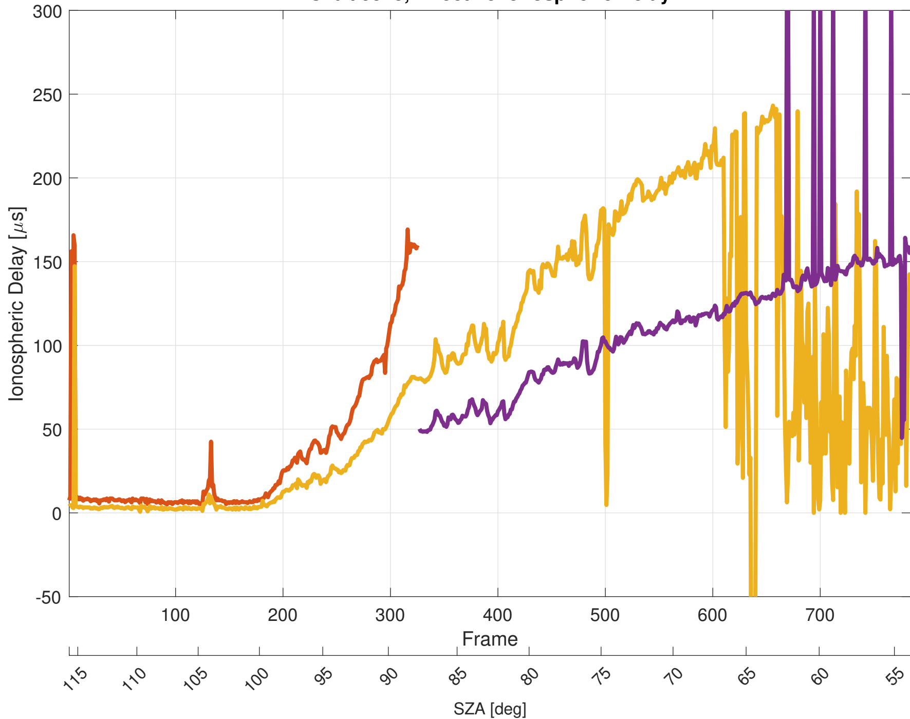
Orbit 9578, Effective Ionospheric Delay
