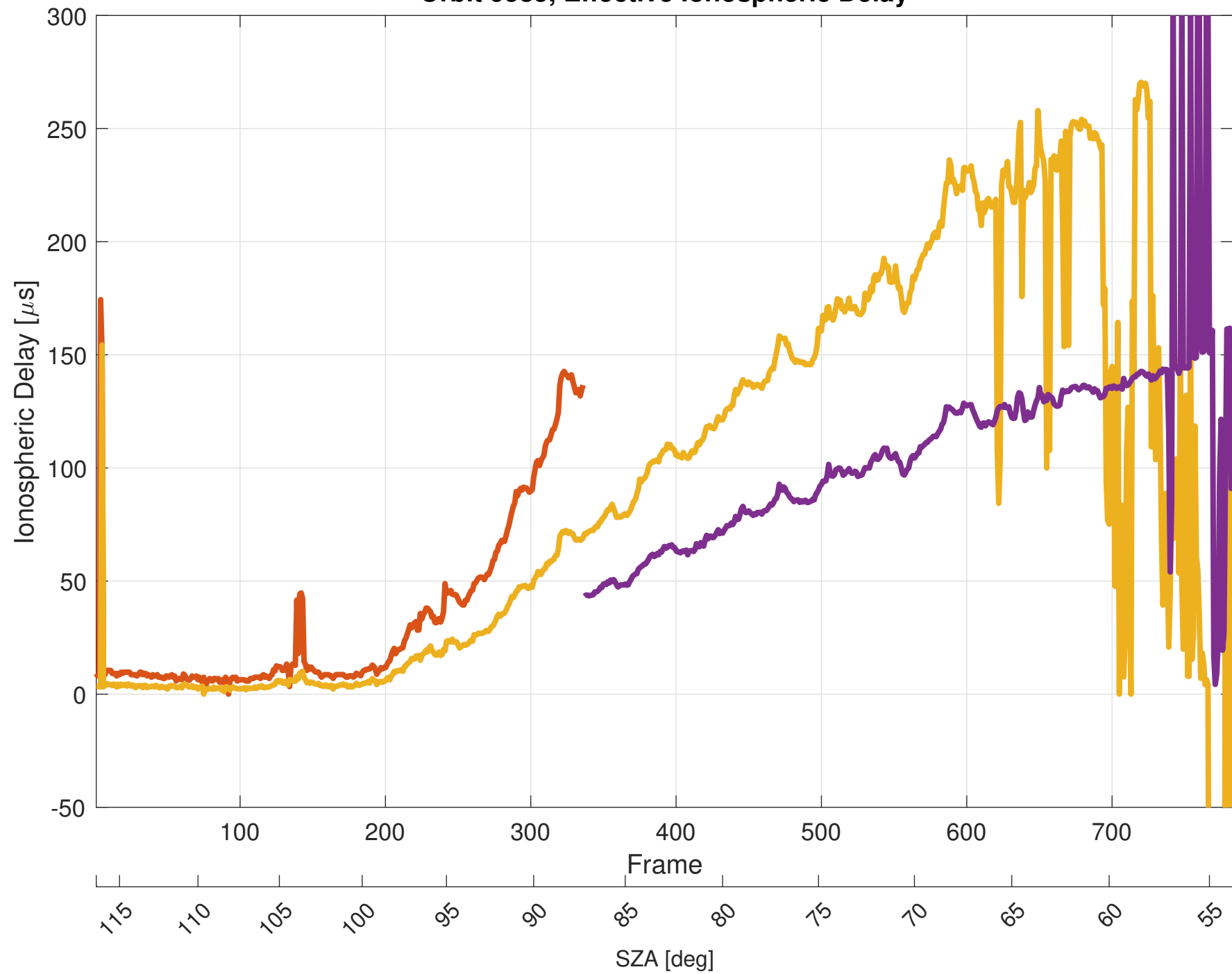
Orbit 9585, Effective Ionospheric Delay
