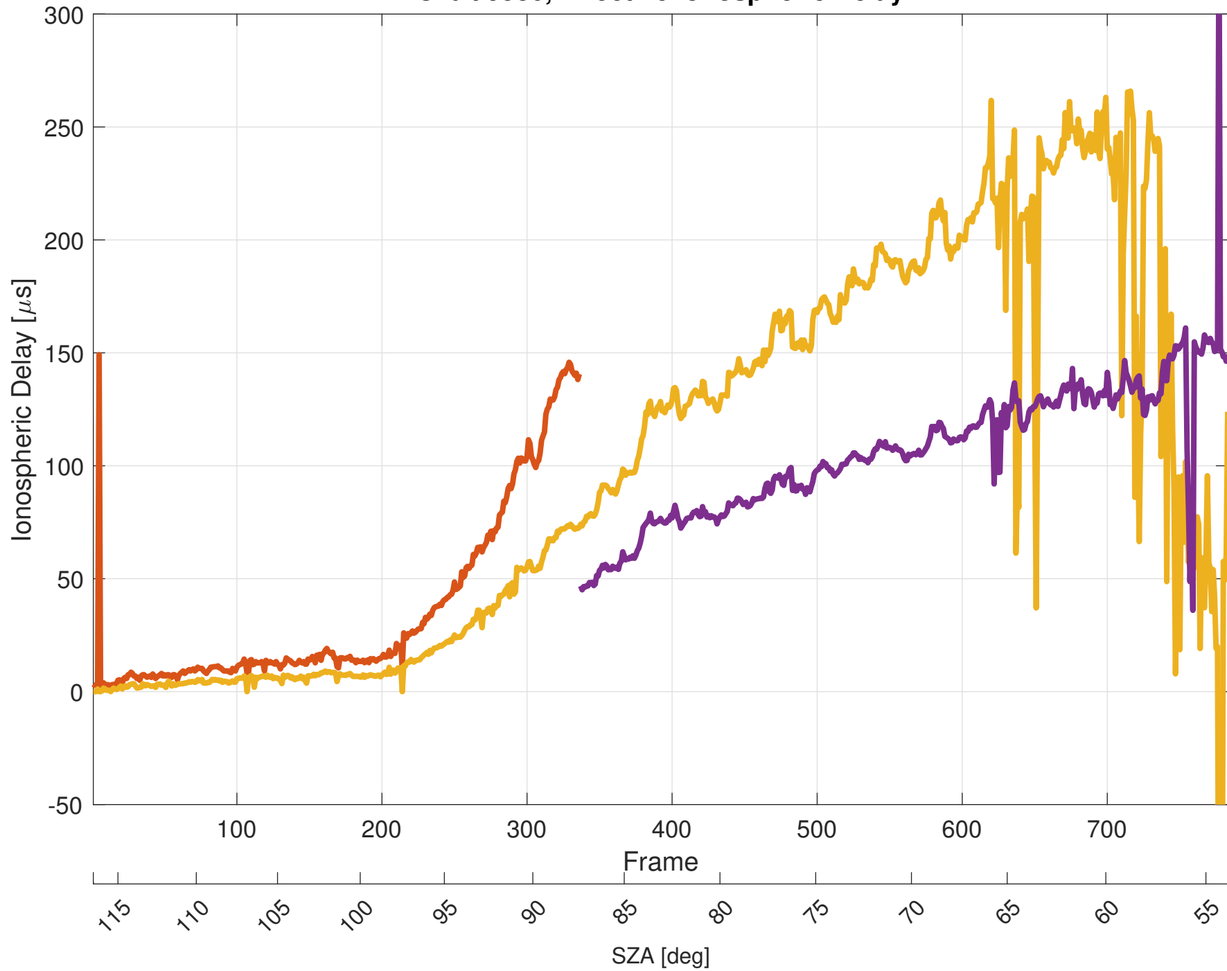
Orbit 9586, Effective Ionospheric Delay
