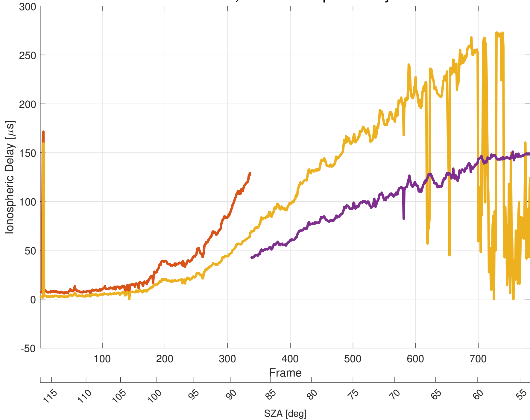
Orbit 9587, Effective Ionospheric Delay
