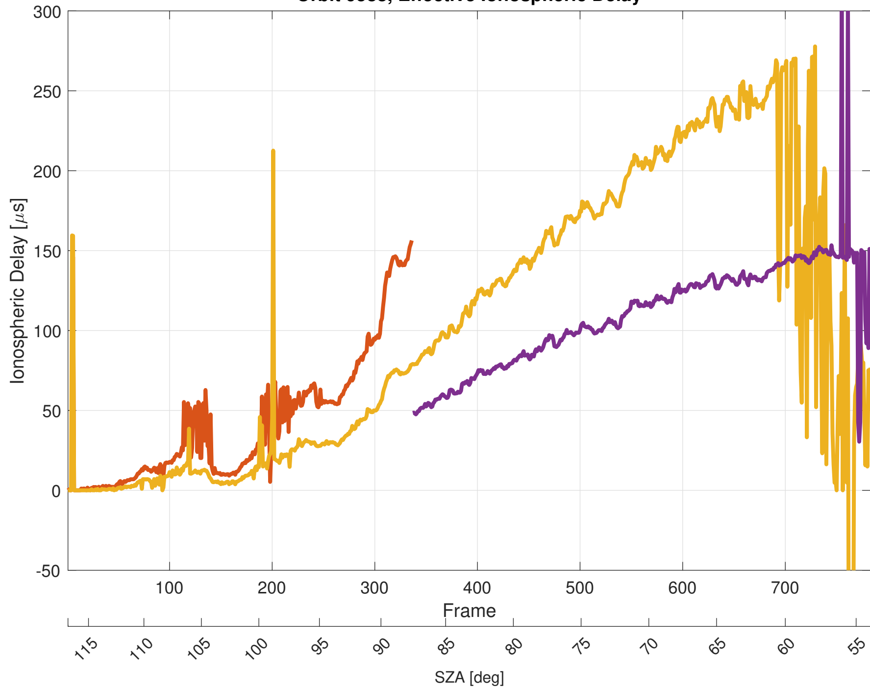
Orbit 9588, Effective Ionospheric Delay
