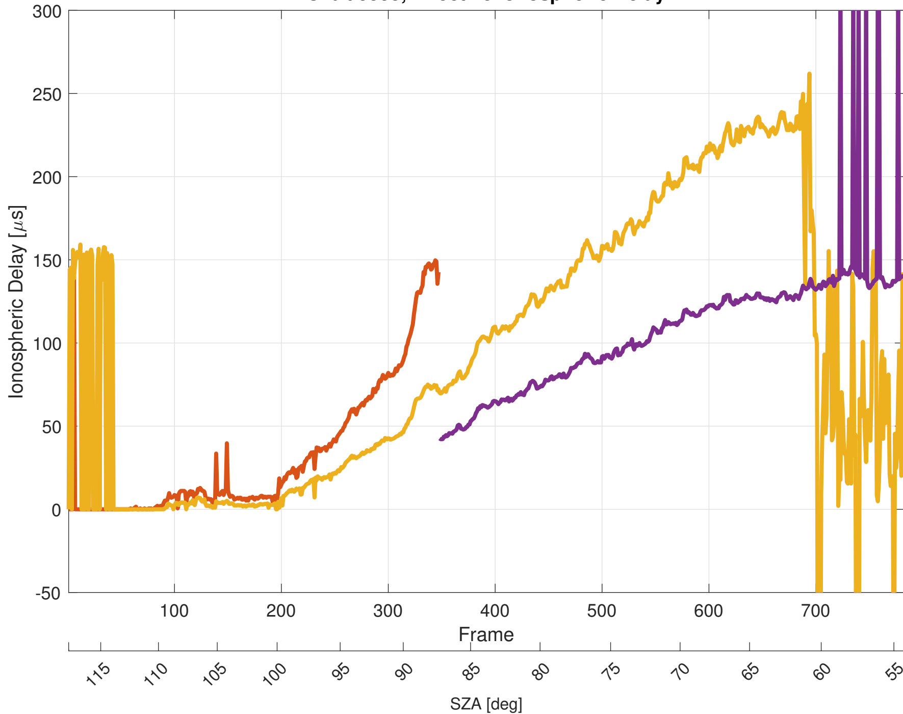
Orbit 9595, Effective Ionospheric Delay
