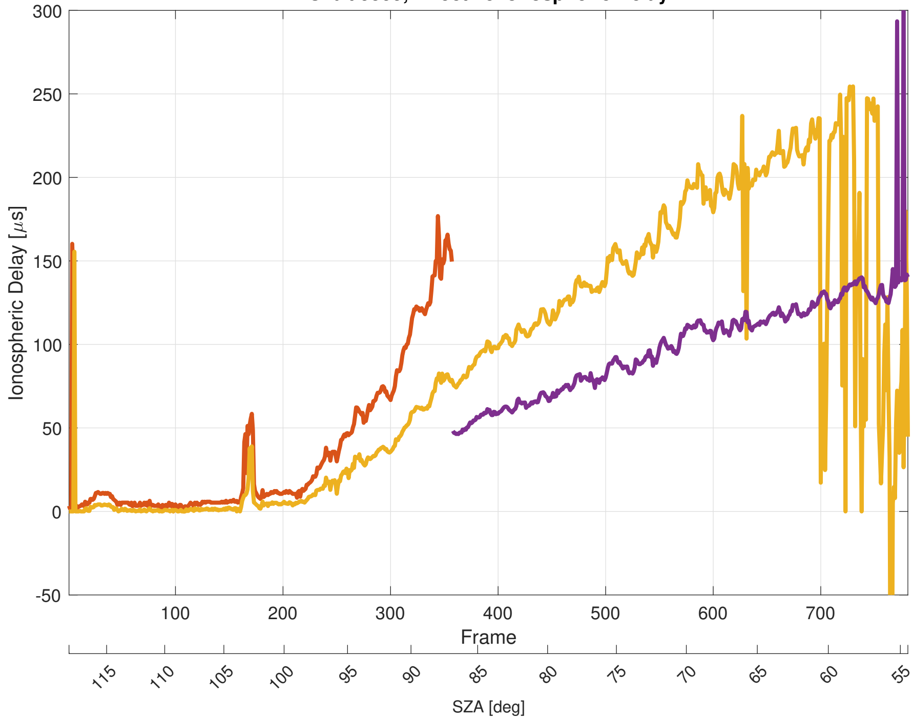
Orbit 9599, Effective Ionospheric Delay
