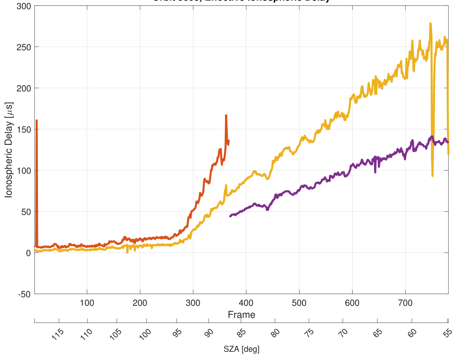
Orbit 9608, Effective Ionospheric Delay
