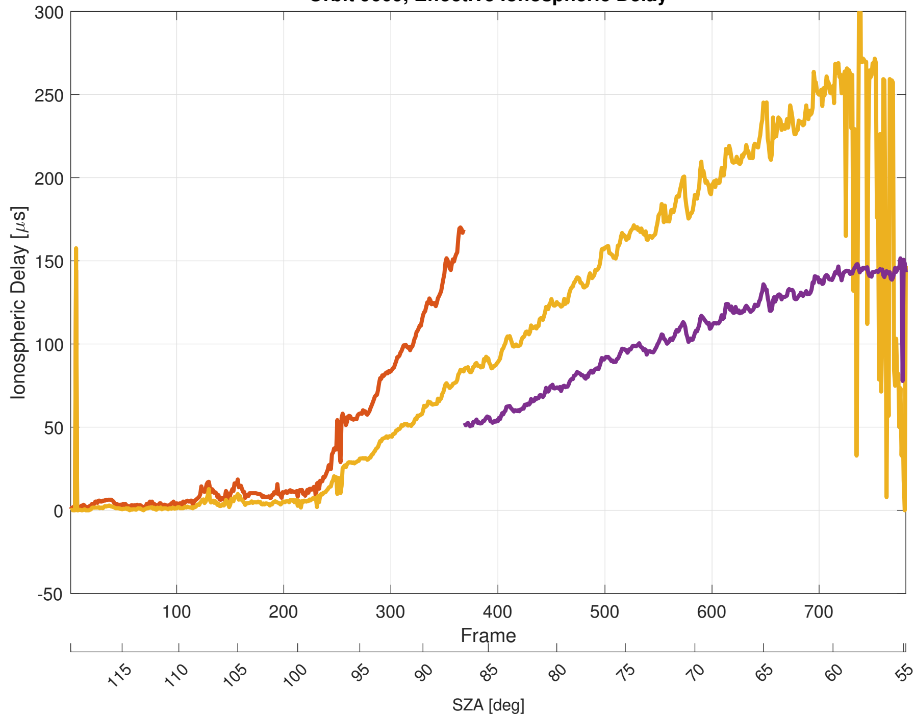
Orbit 9609, Effective Ionospheric Delay
