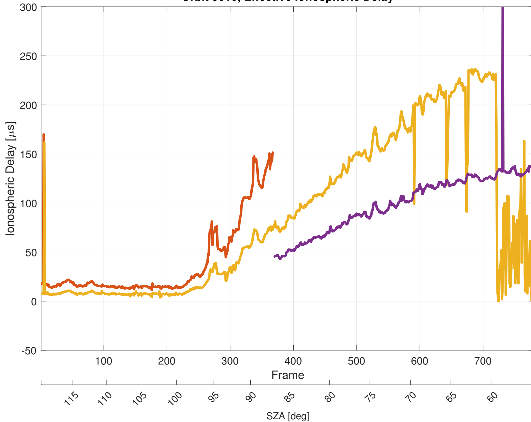
Orbit 9610, Effective Ionospheric Delay
