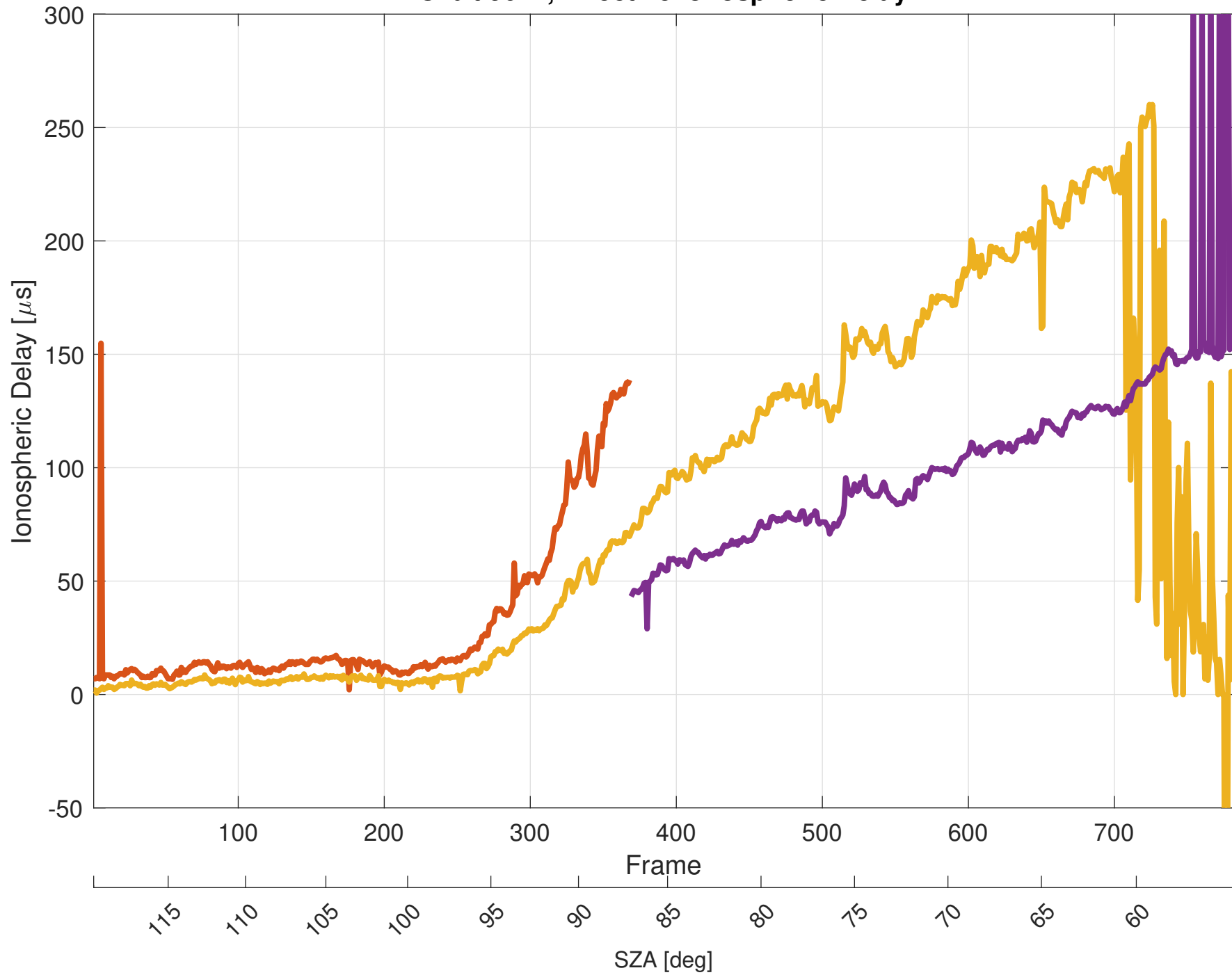
Orbit 9611, Effective Ionospheric Delay
