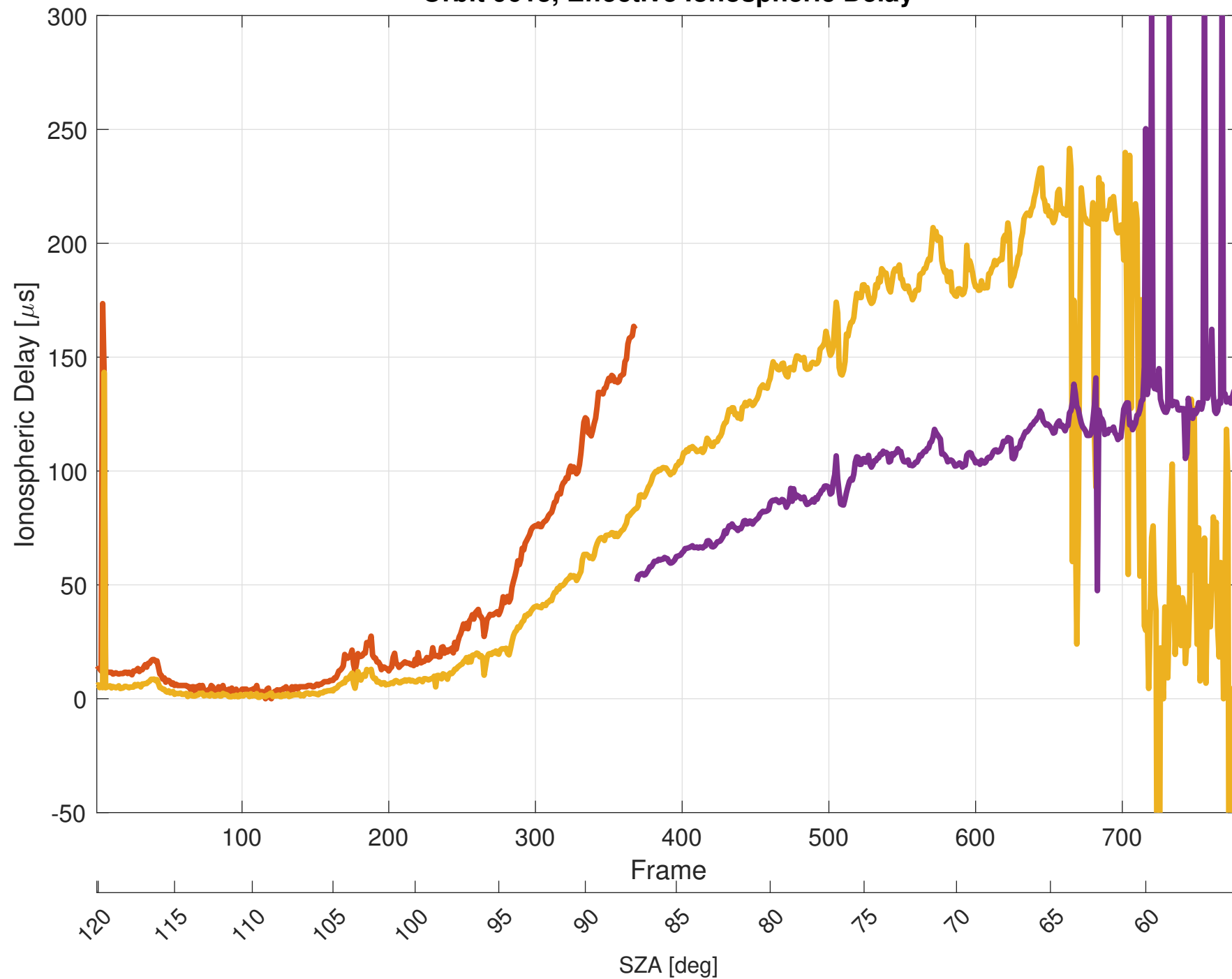
Orbit 9613, Effective Ionospheric Delay
