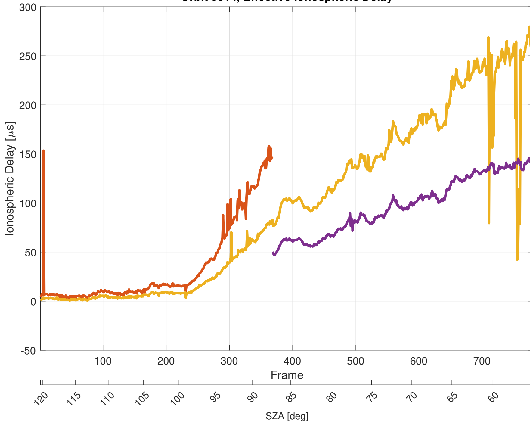
Orbit 9614, Effective Ionospheric Delay
