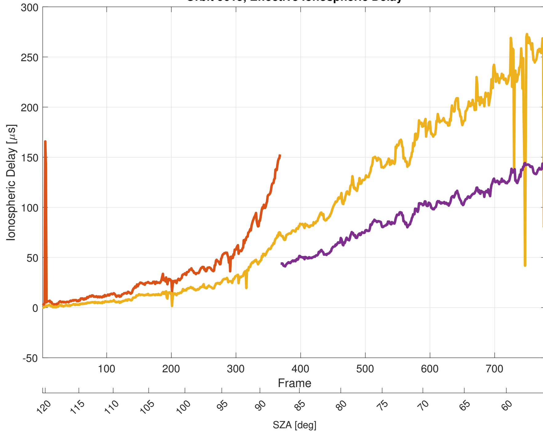
Orbit 9615, Effective Ionospheric Delay
