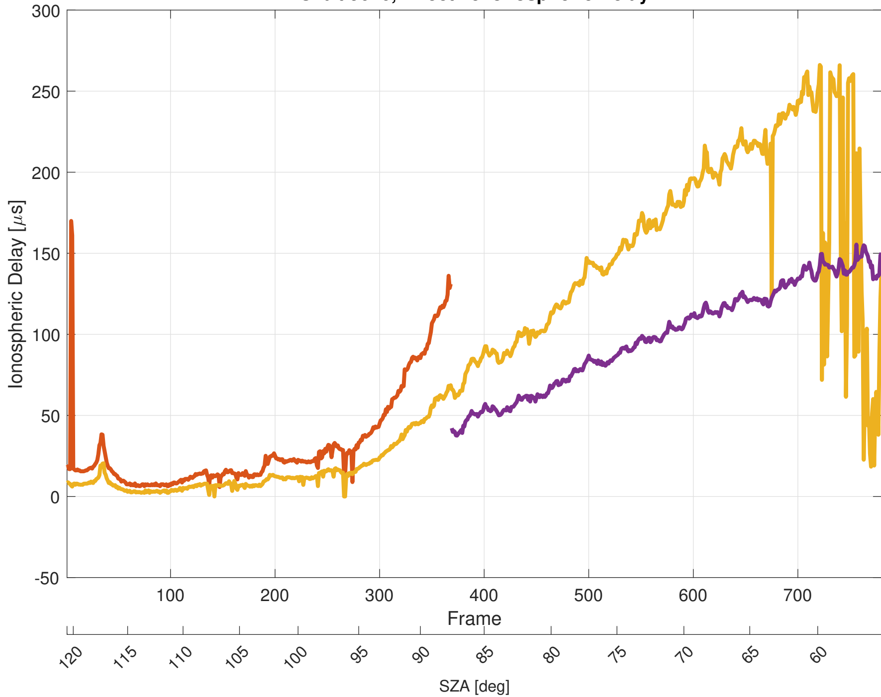
Orbit 9616, Effective Ionospheric Delay
