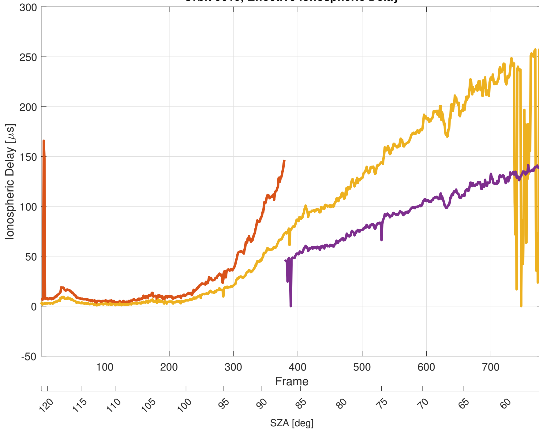
Orbit 9619, Effective Ionospheric Delay
