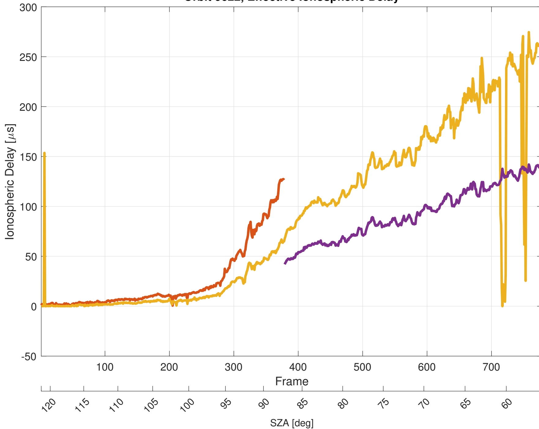
Orbit 9622, Effective Ionospheric Delay
