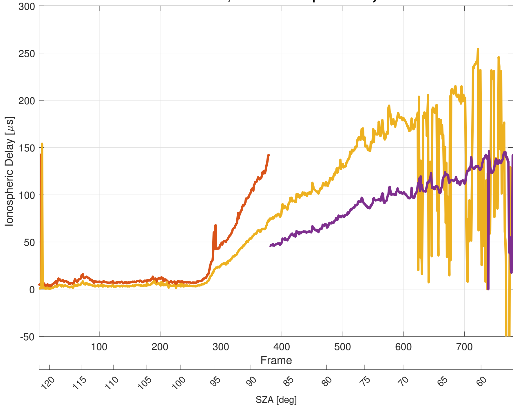
Orbit 9624, Effective Ionospheric Delay
