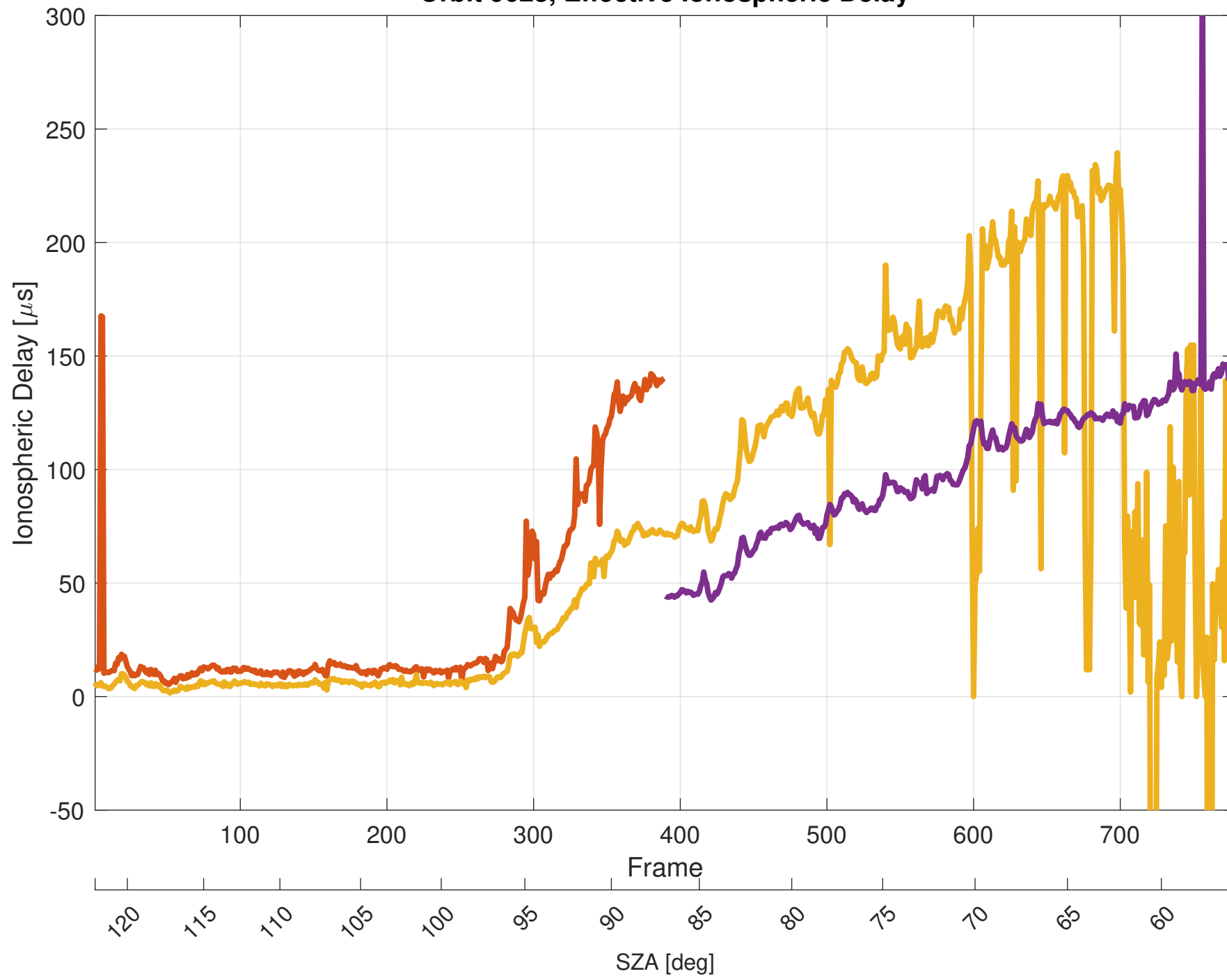
Orbit 9628, Effective Ionospheric Delay
