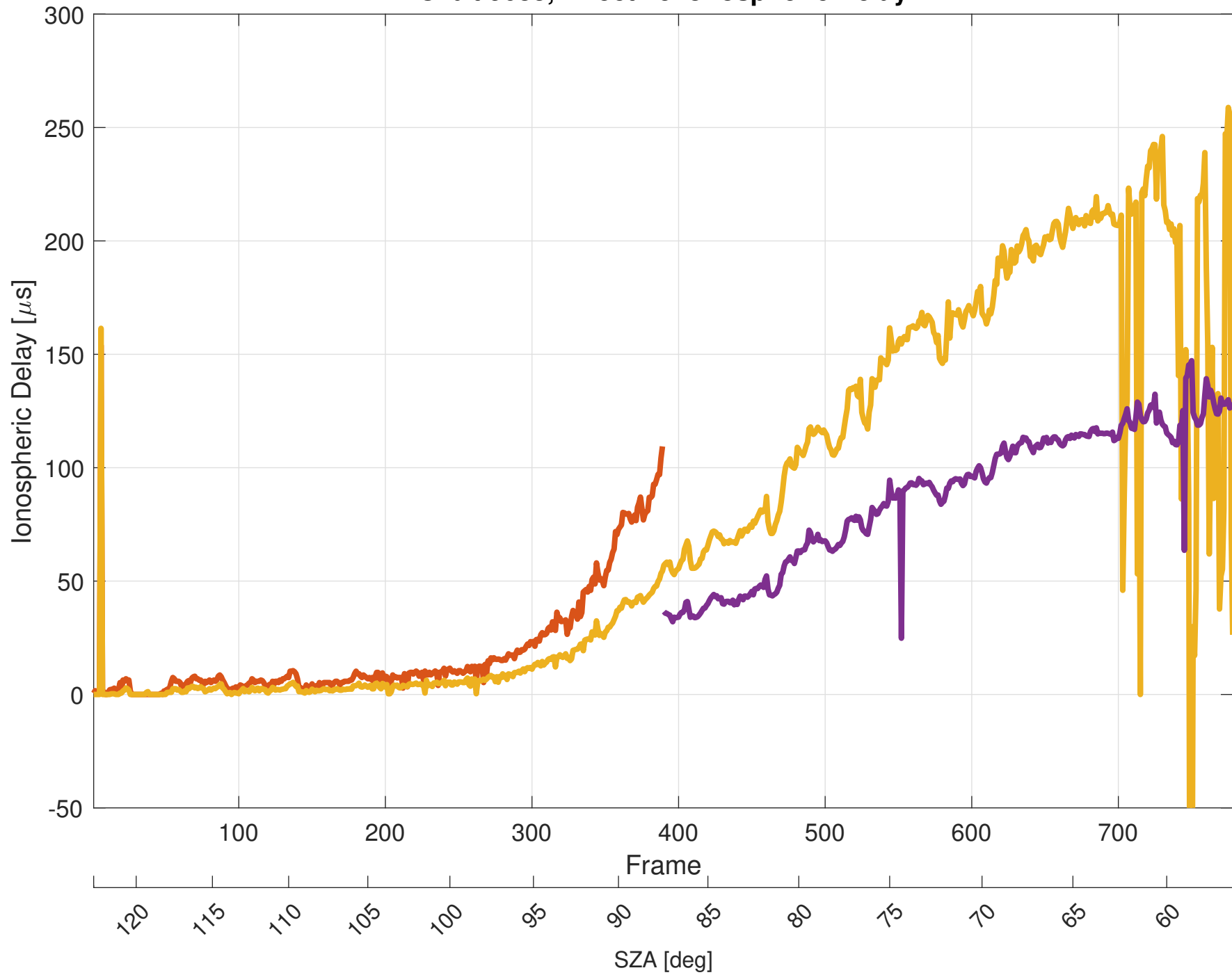
Orbit 9633, Effective Ionospheric Delay
