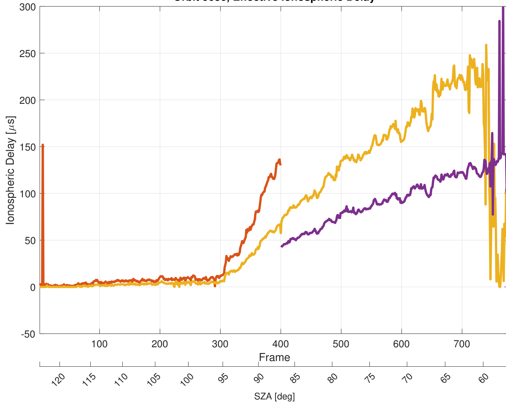
Orbit 9636, Effective Ionospheric Delay
