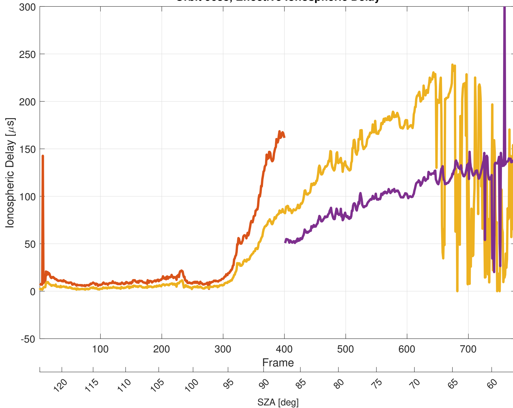
Orbit 9638, Effective Ionospheric Delay
