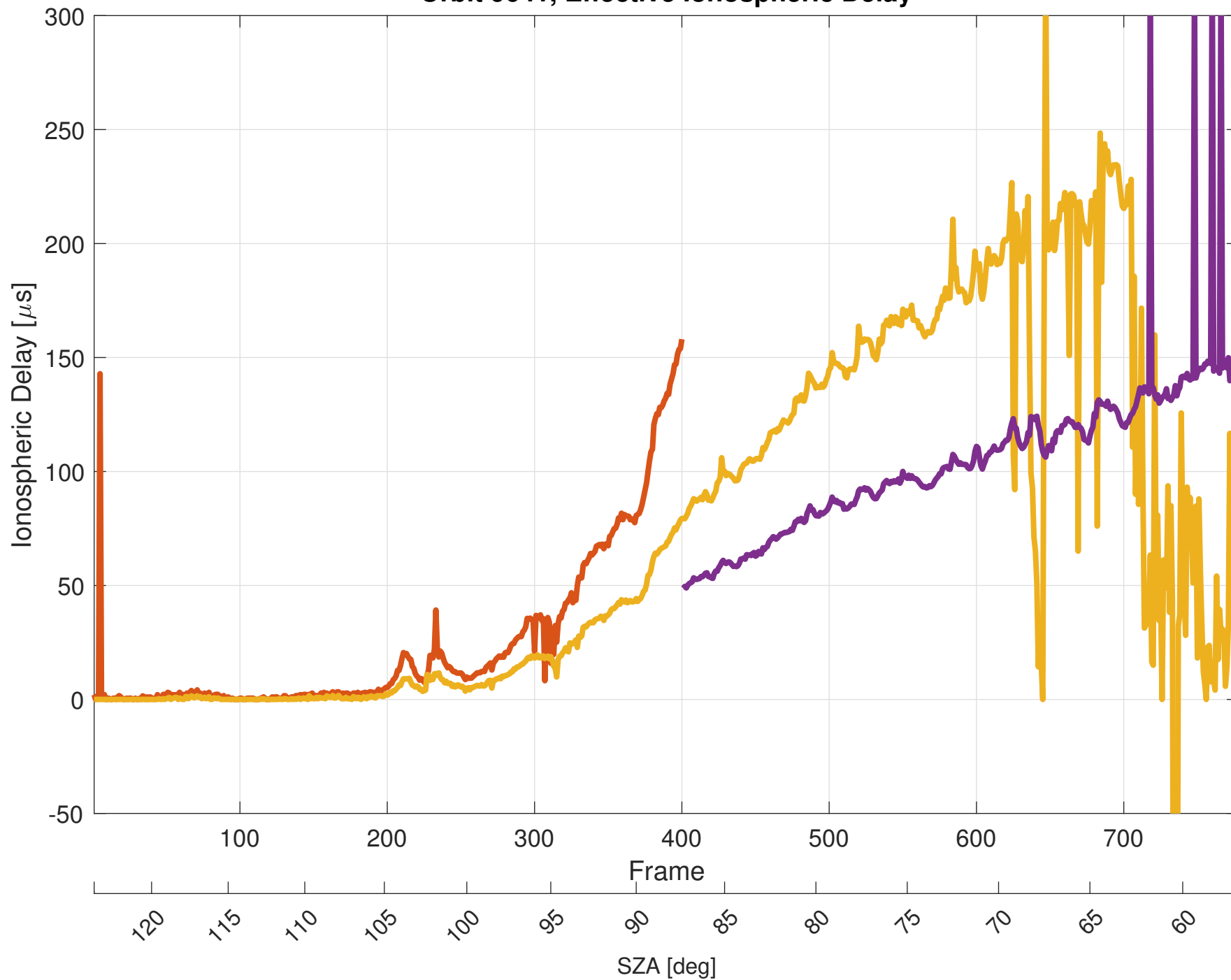
Orbit 9641, Effective Ionospheric Delay
