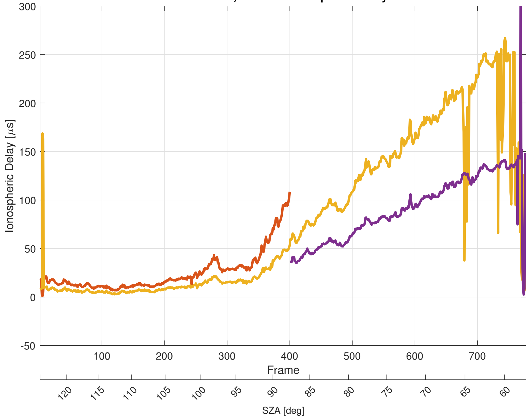
Orbit 9643, Effective Ionospheric Delay
