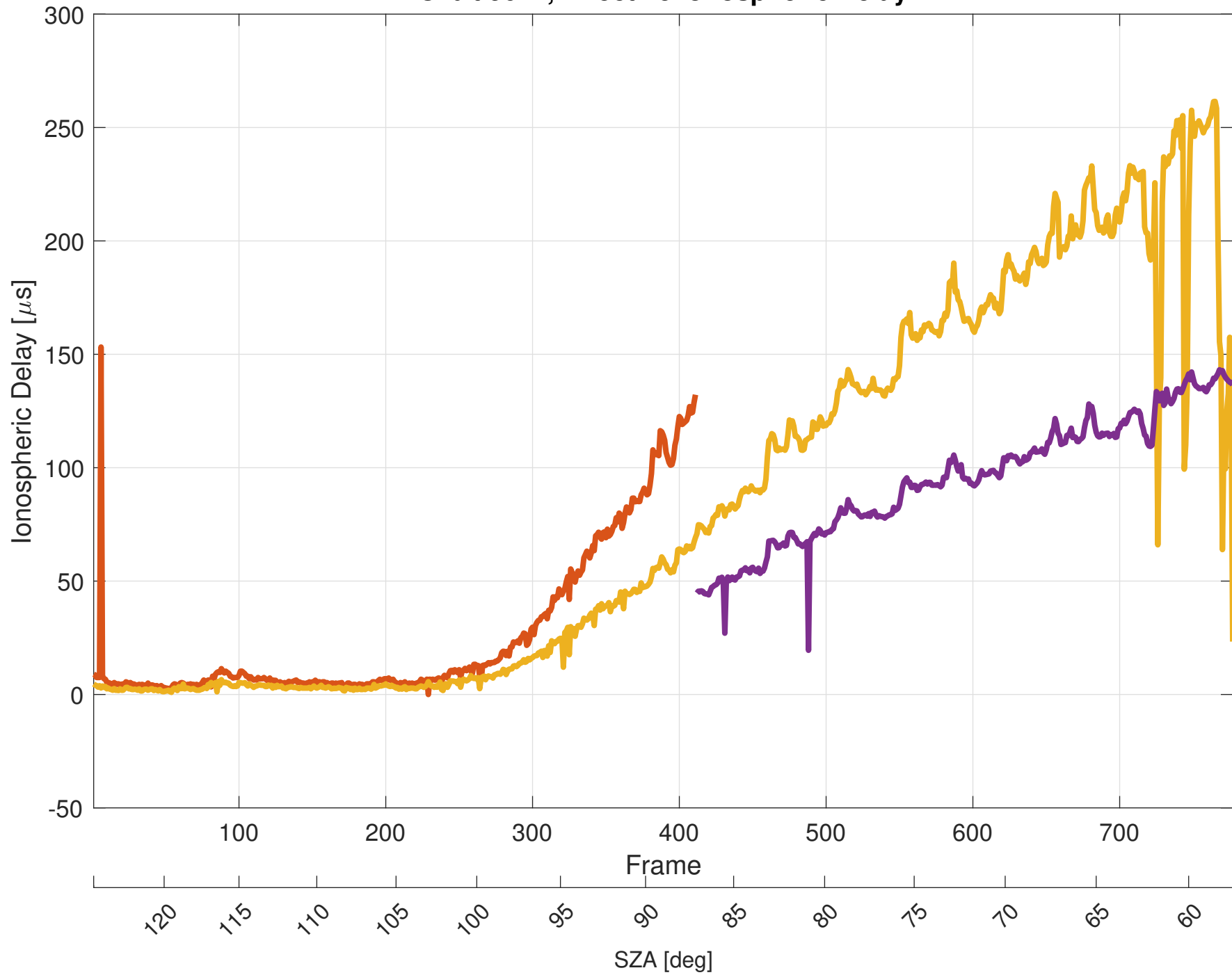
Orbit 9647, Effective Ionospheric Delay
