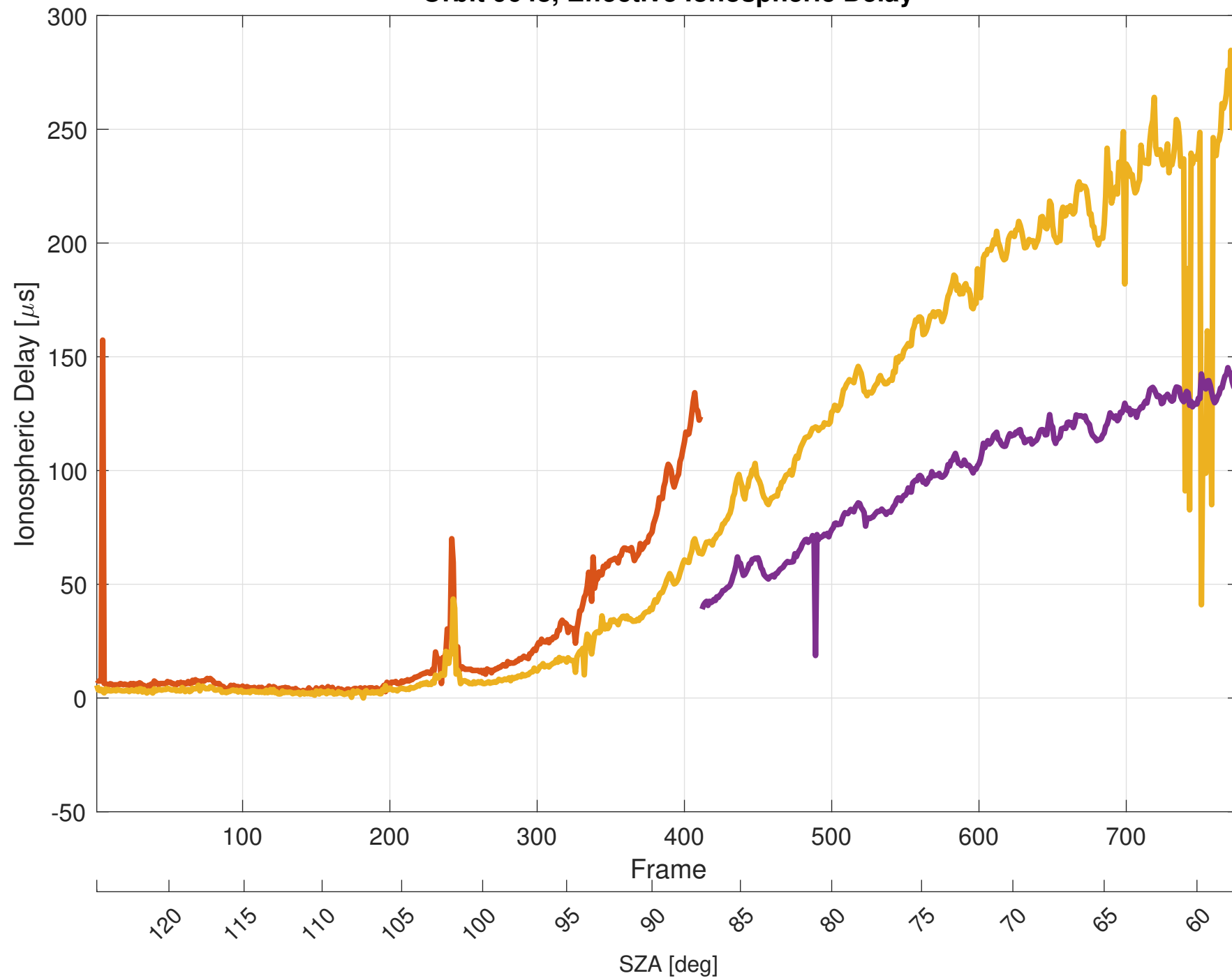
Orbit 9648, Effective Ionospheric Delay
