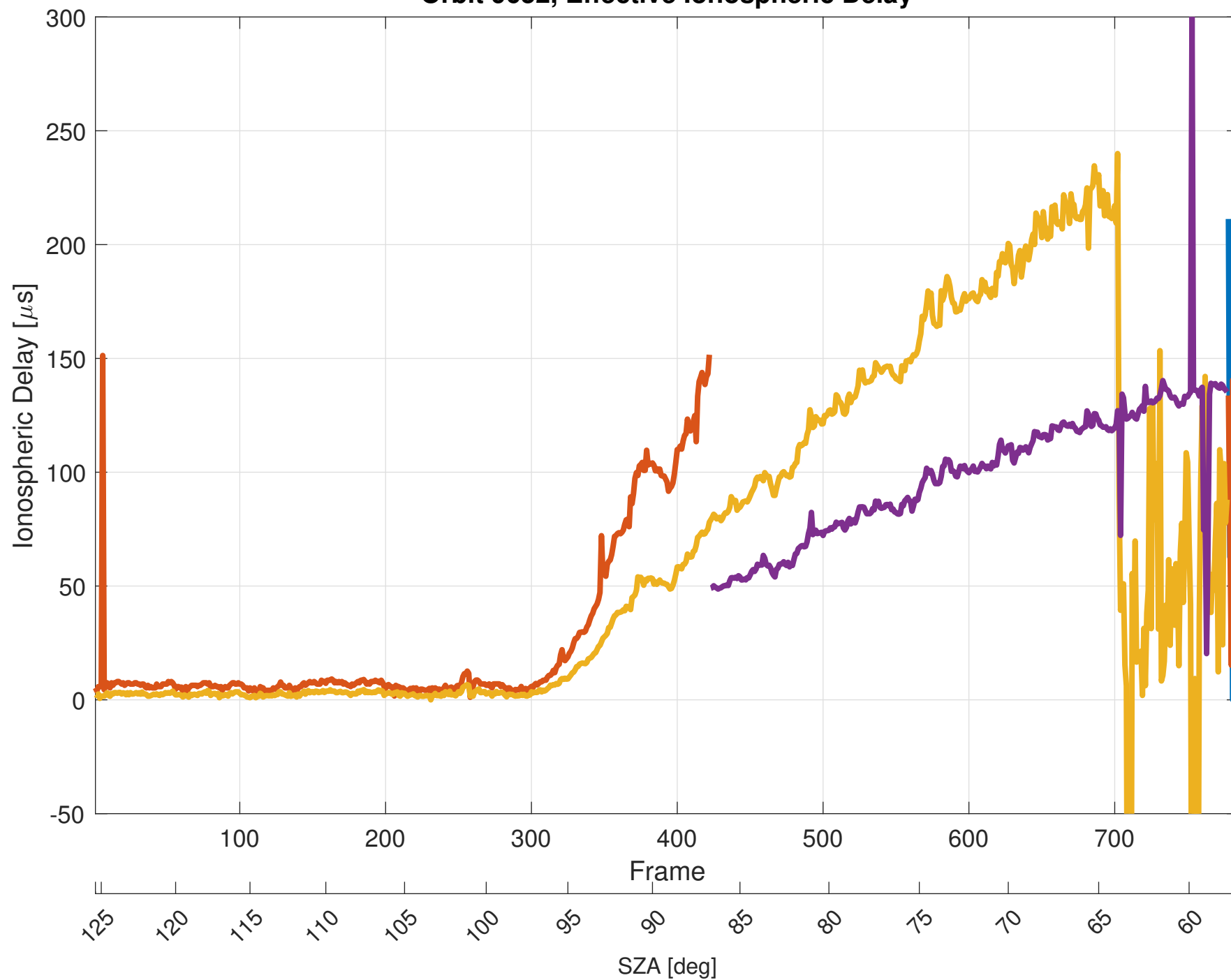
Orbit 9652, Effective Ionospheric Delay
