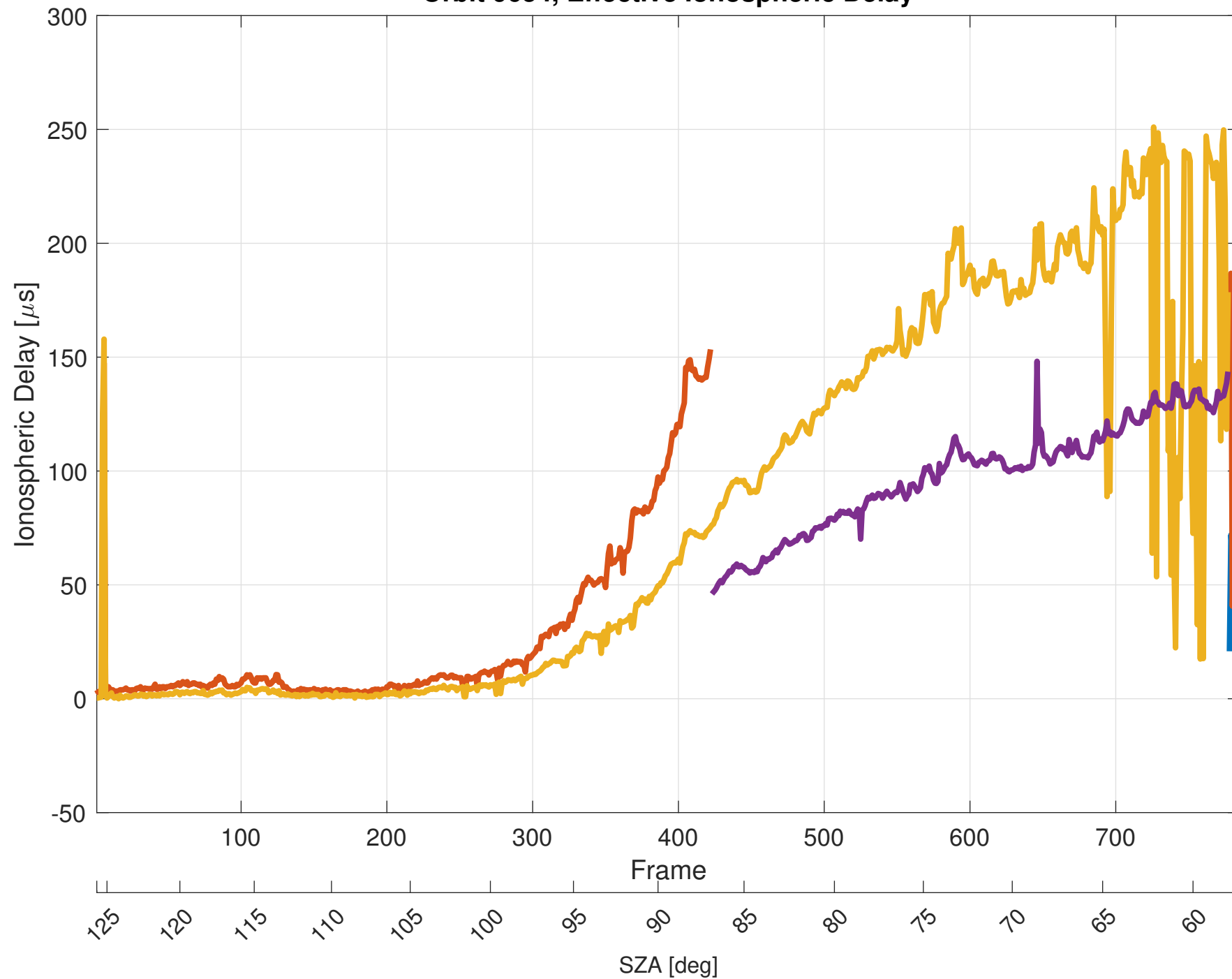
Orbit 9654, Effective Ionospheric Delay
