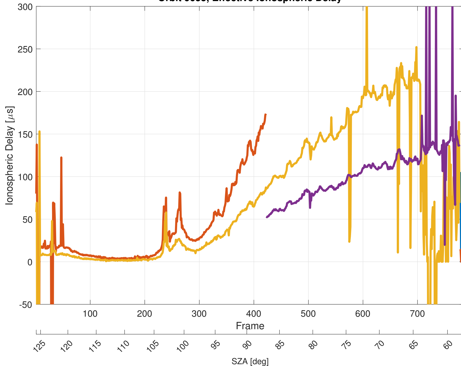
Orbit 9655, Effective Ionospheric Delay
