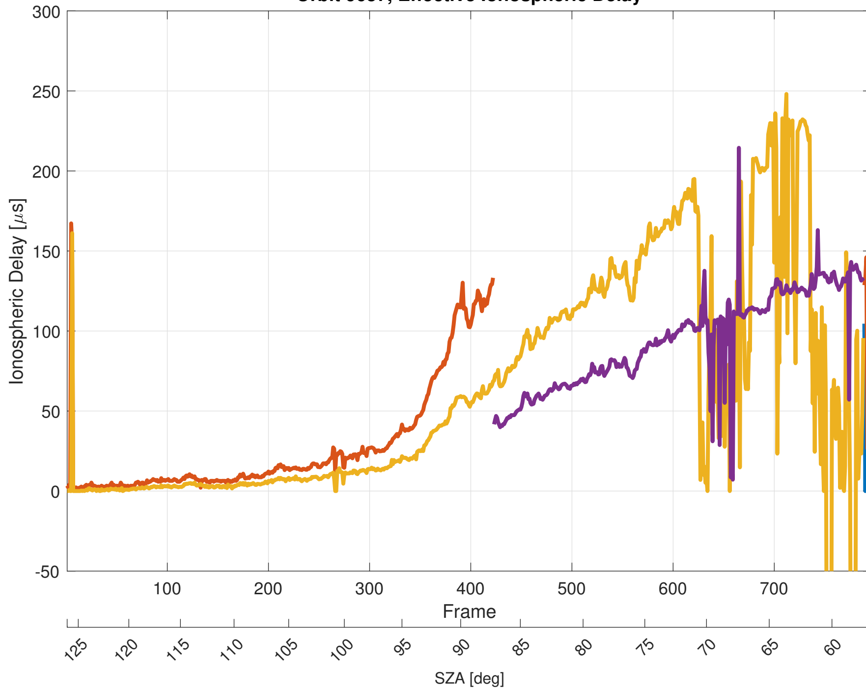
Orbit 9657, Effective Ionospheric Delay
