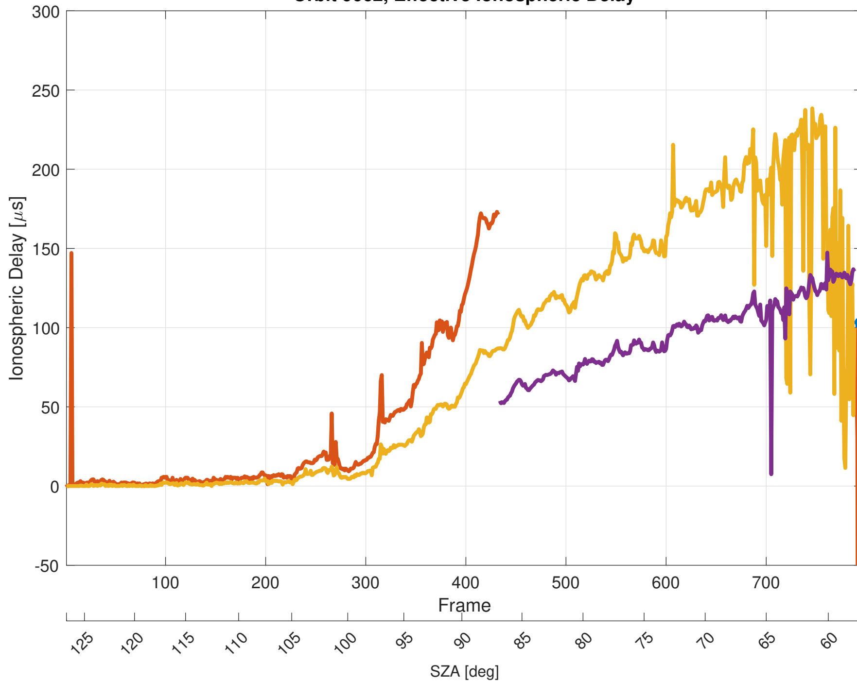
Orbit 9662, Effective Ionospheric Delay
