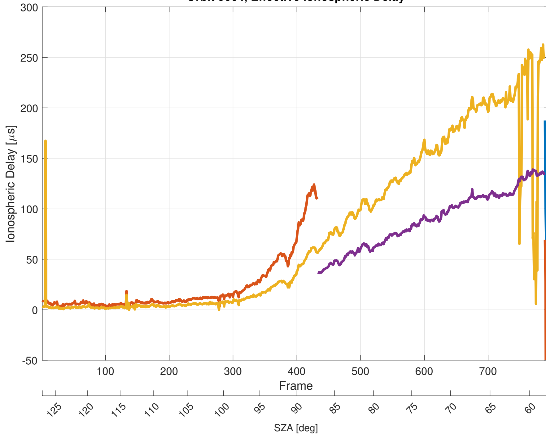
Orbit 9664, Effective Ionospheric Delay
