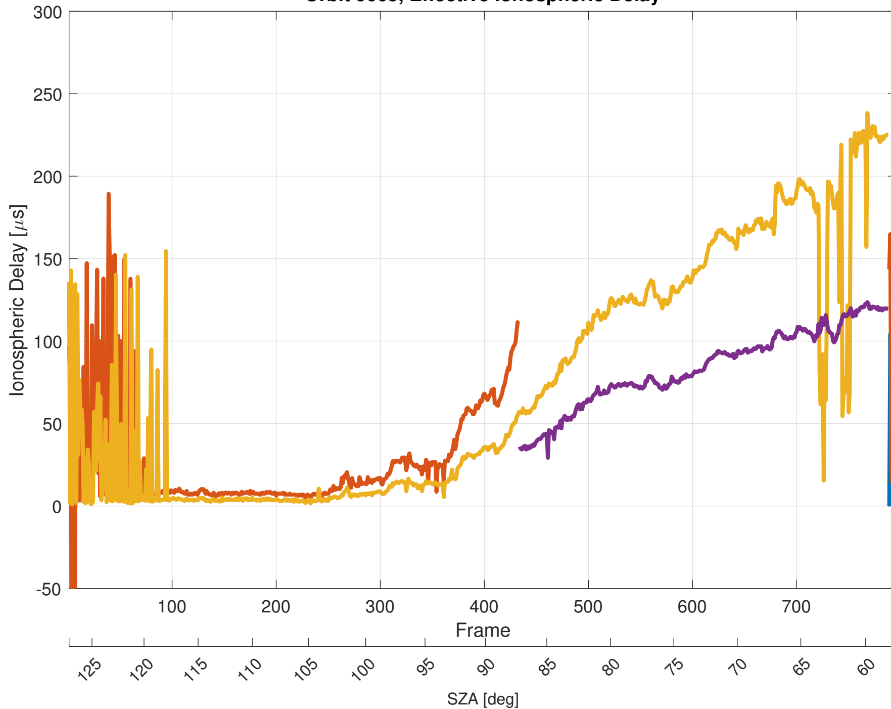
Orbit 9665, Effective Ionospheric Delay
