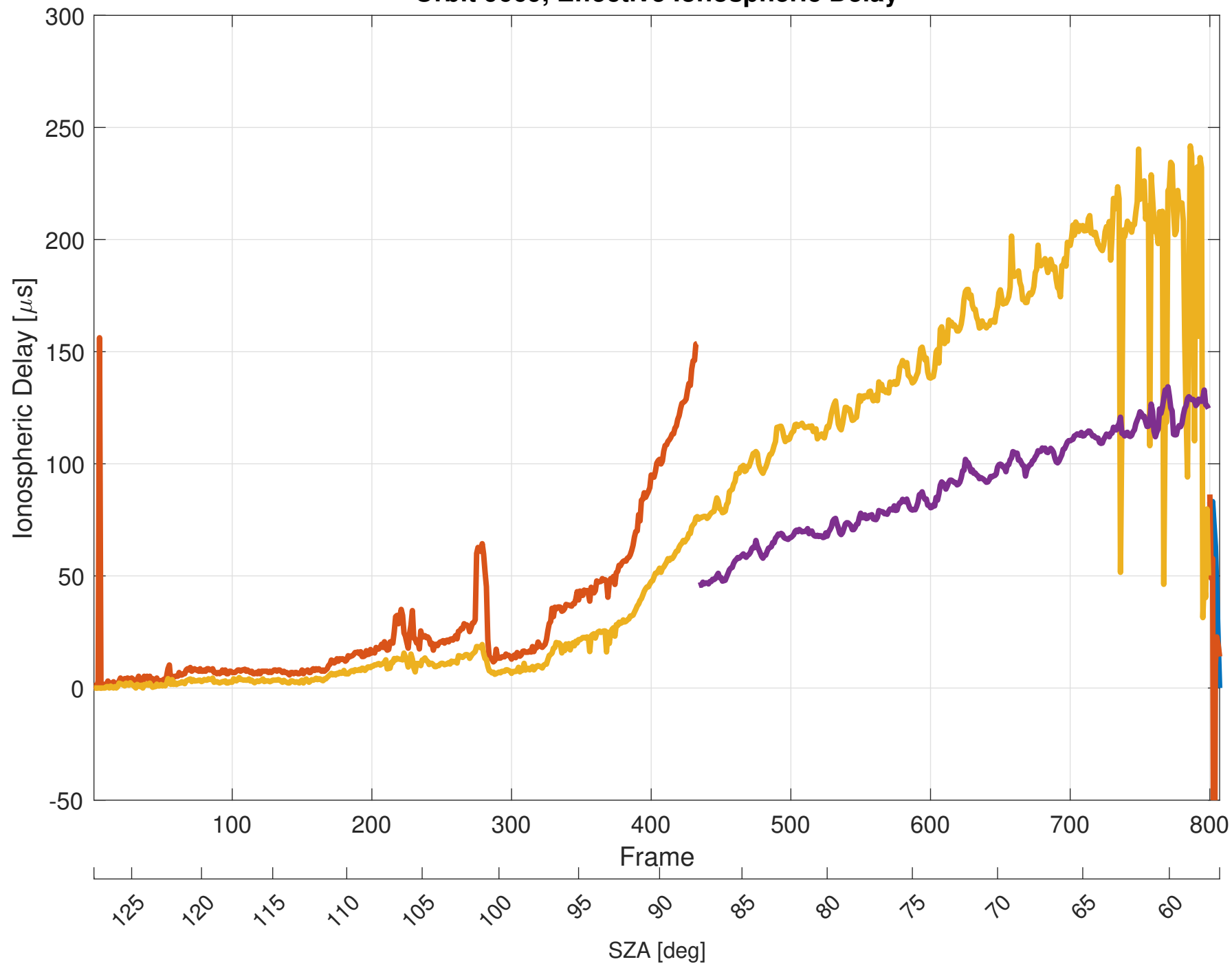
Orbit 9669, Effective Ionospheric Delay
