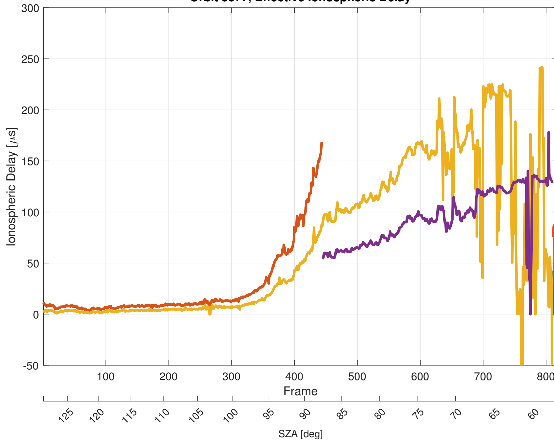
Orbit 9677, Effective Ionospheric Delay
