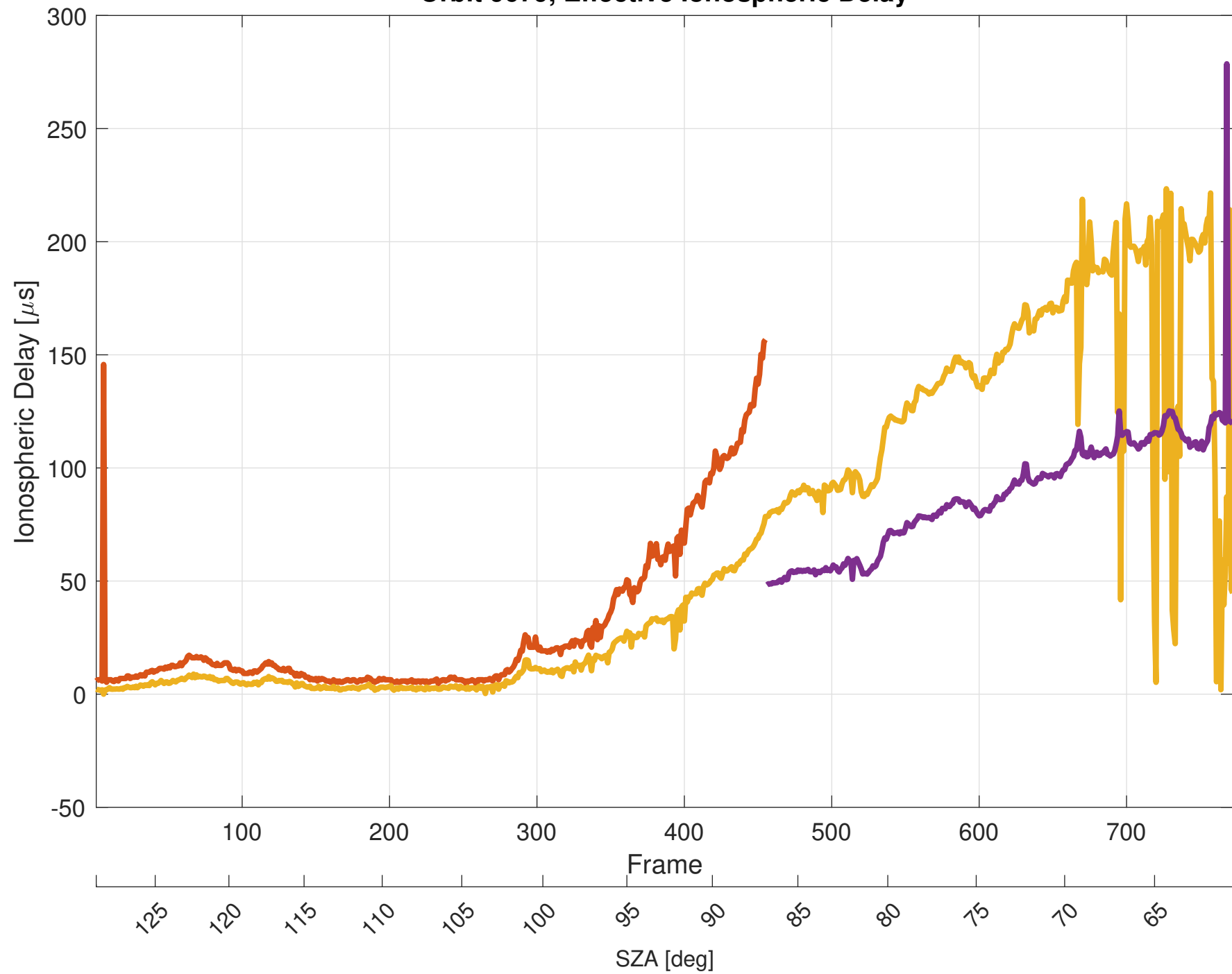
Orbit 9679, Effective Ionospheric Delay
