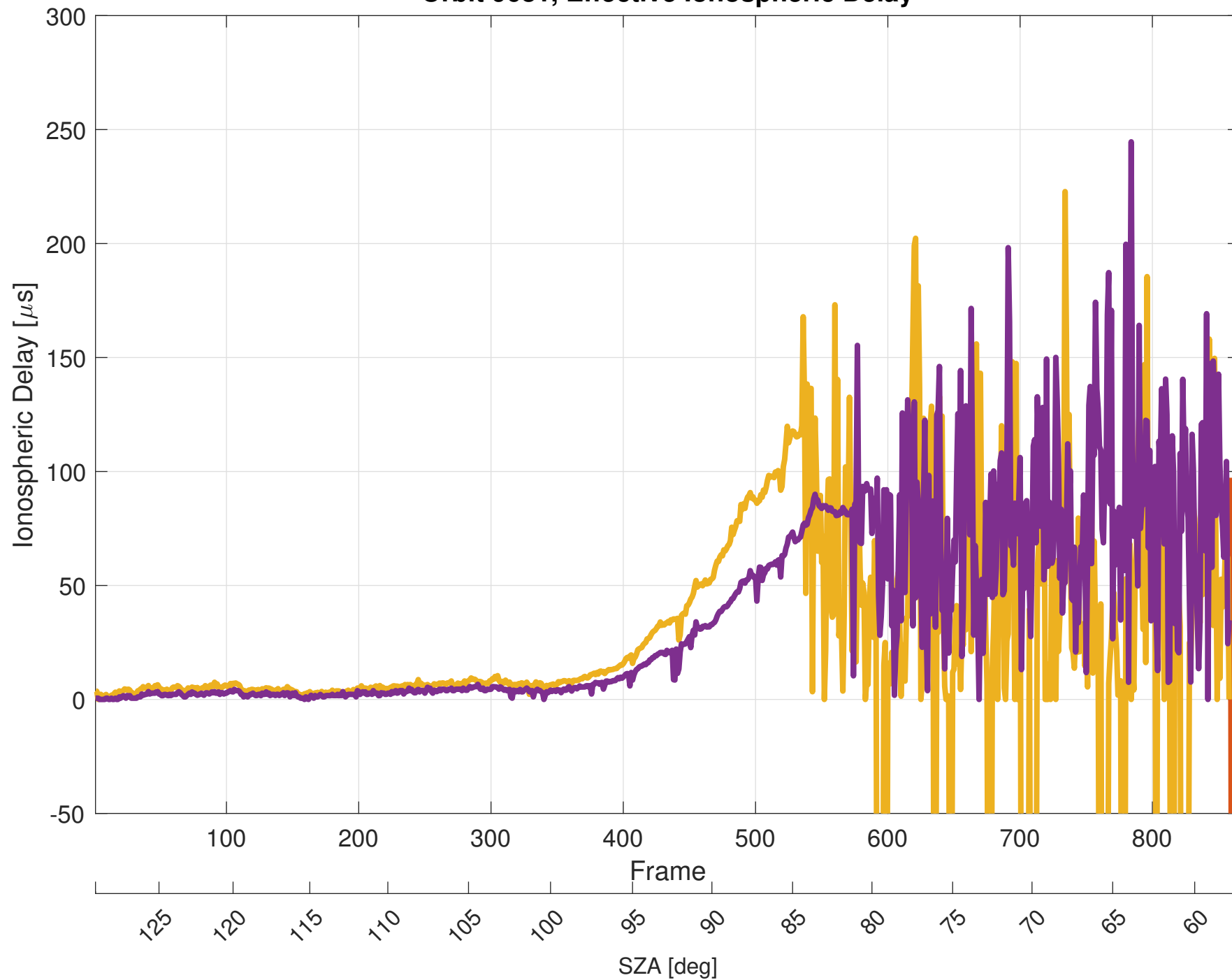
Orbit 9681, Effective Ionospheric Delay
