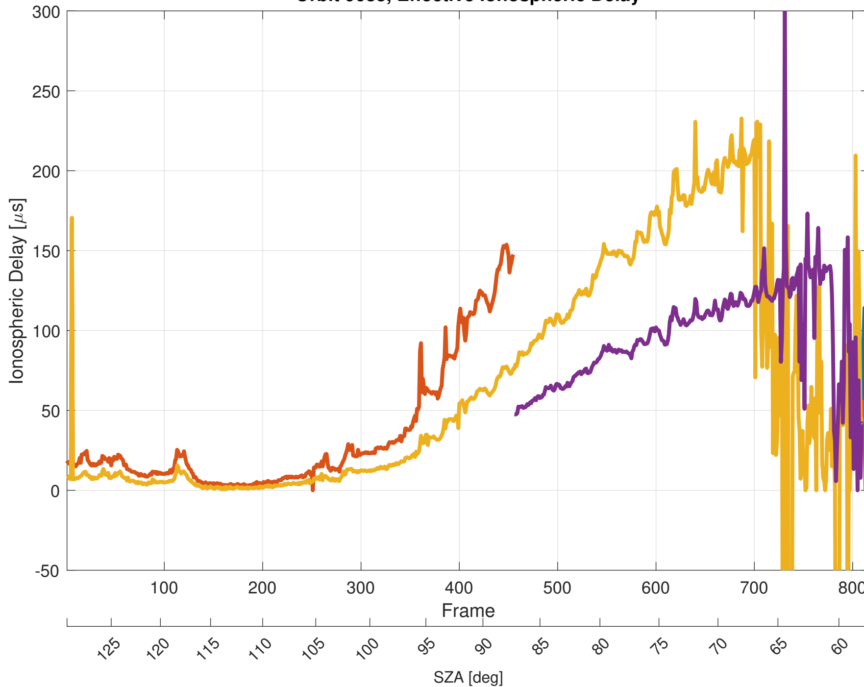
Orbit 9683, Effective Ionospheric Delay
