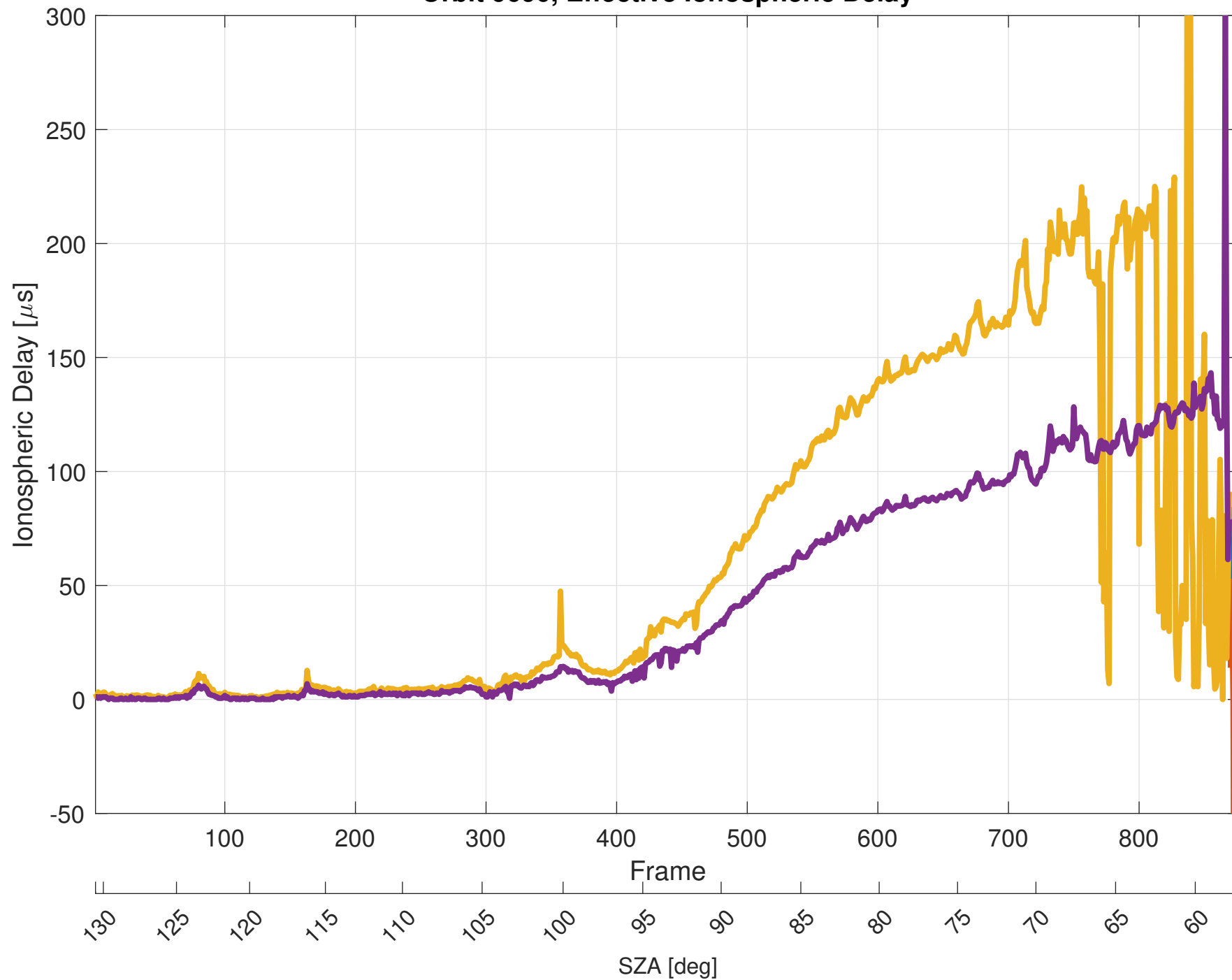
Orbit 9690, Effective Ionospheric Delay
