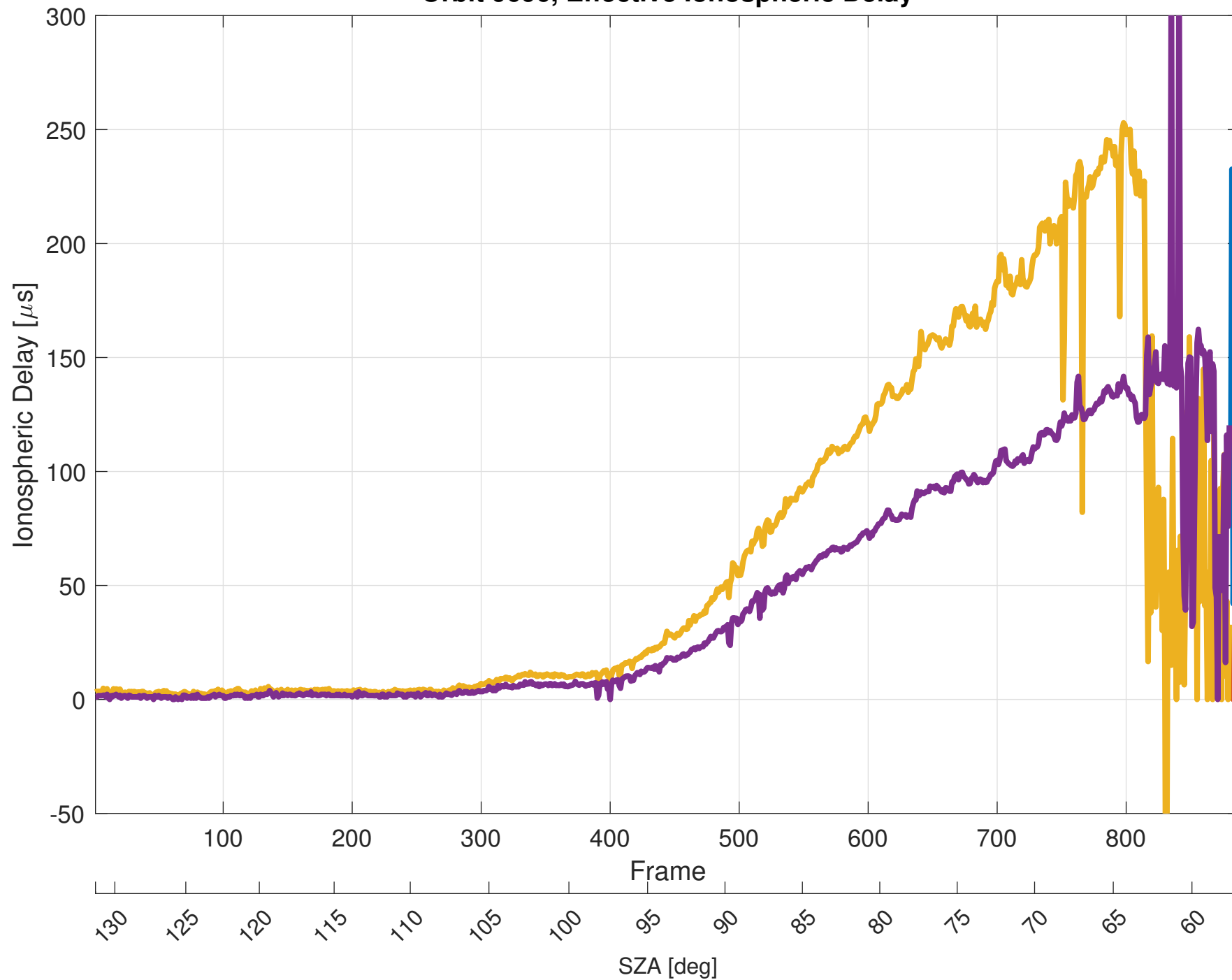
Orbit 9696, Effective Ionospheric Delay
