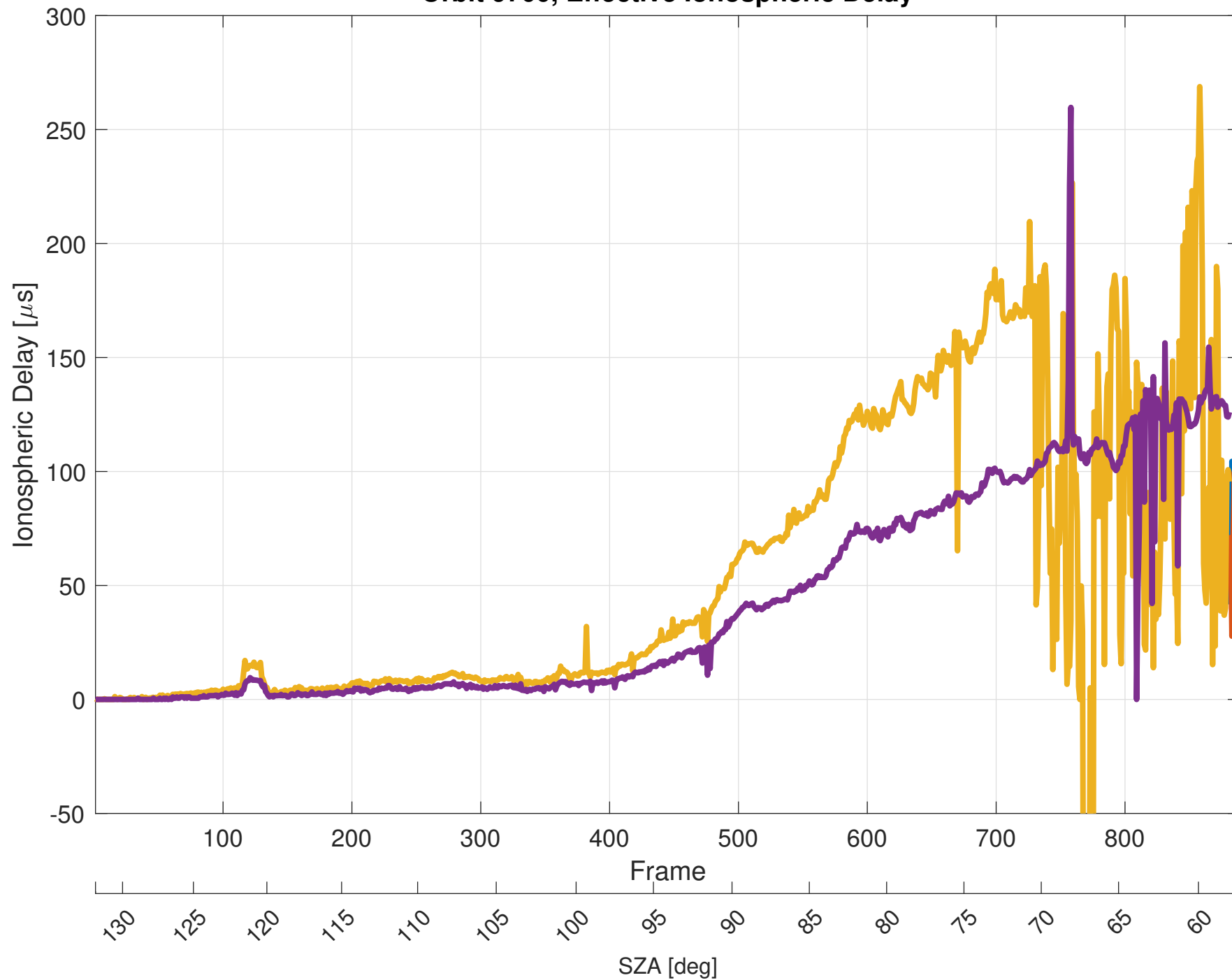
Orbit 9700, Effective Ionospheric Delay
