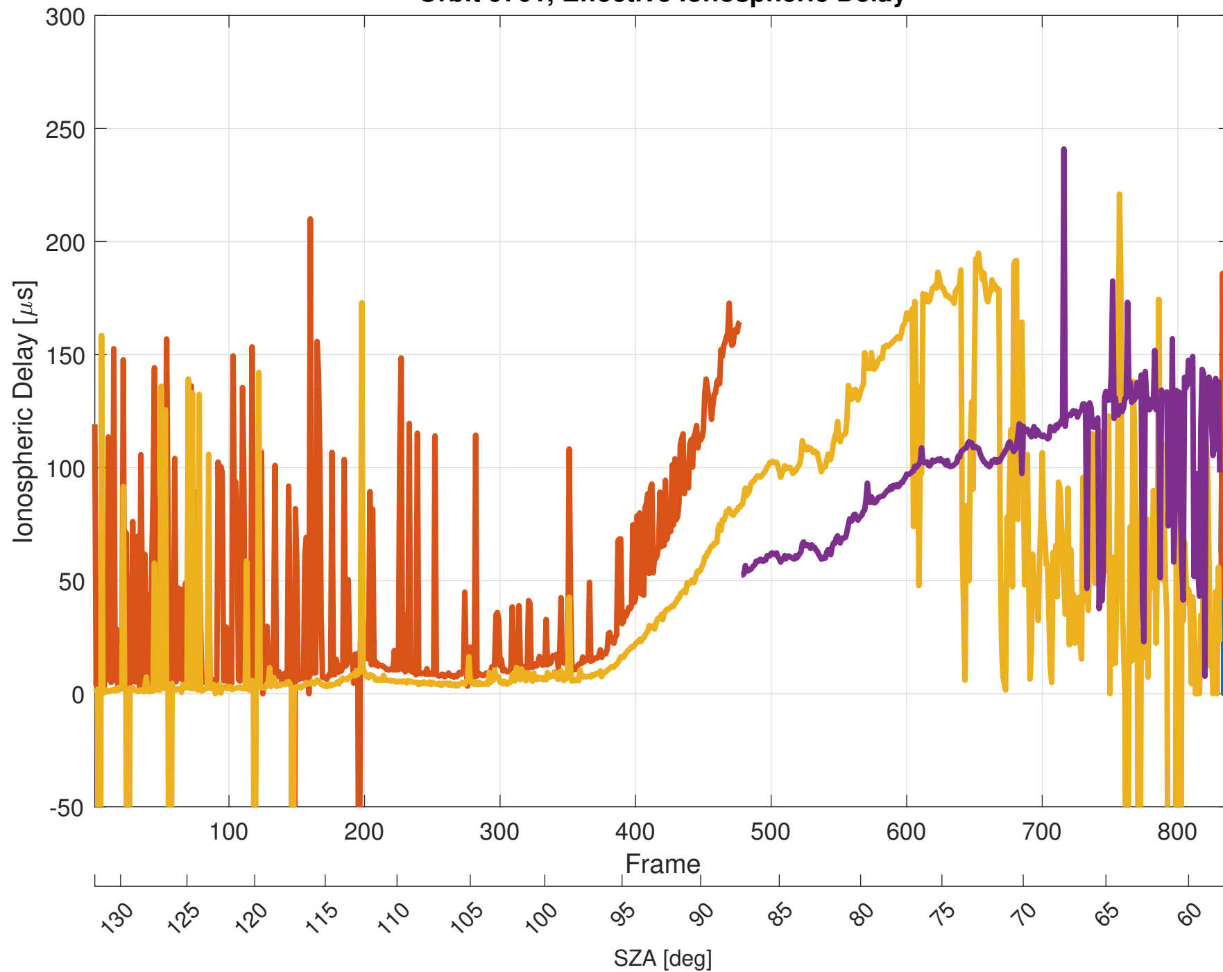
Orbit 9701, Effective Ionospheric Delay
