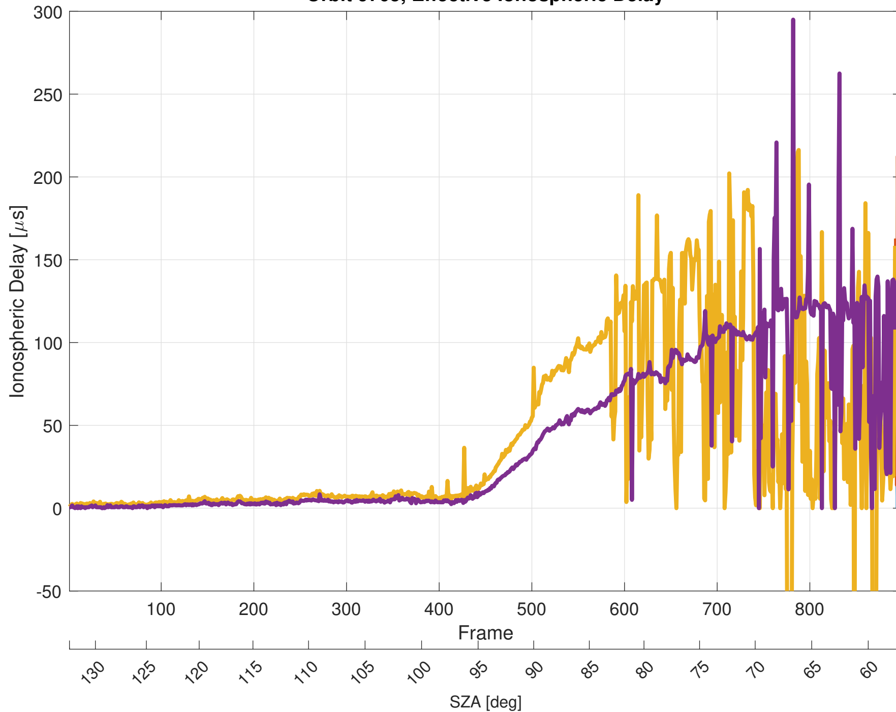
Orbit 9705, Effective Ionospheric Delay
