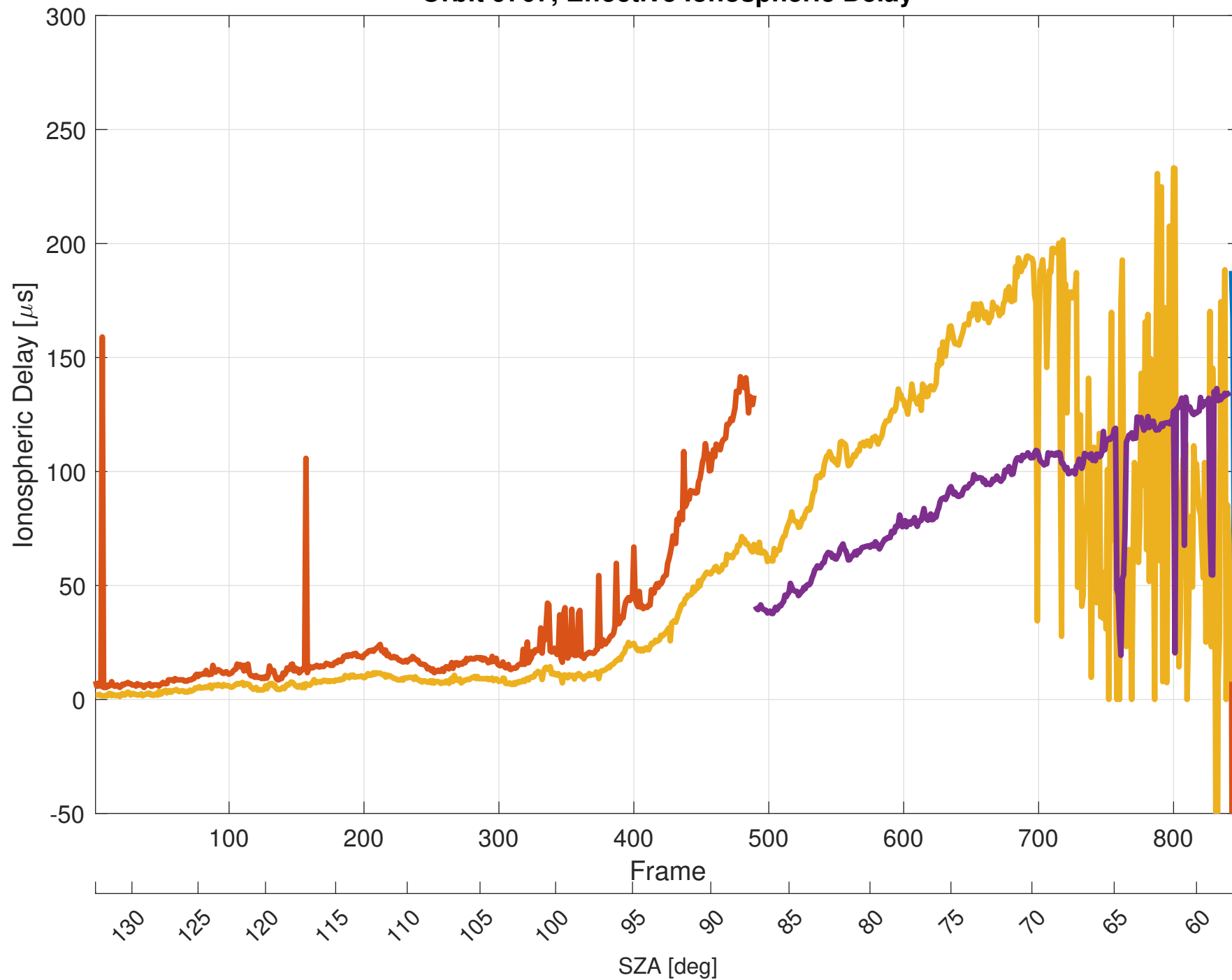
Orbit 9707, Effective Ionospheric Delay
