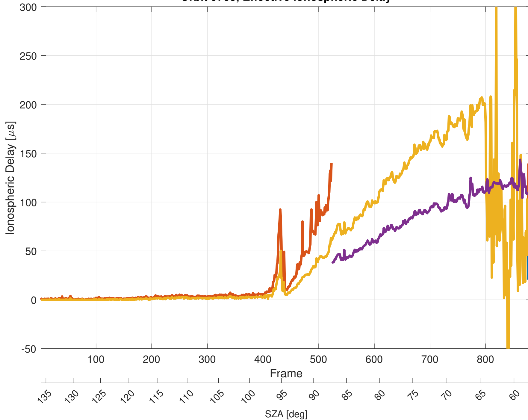
Orbit 9733, Effective Ionospheric Delay
