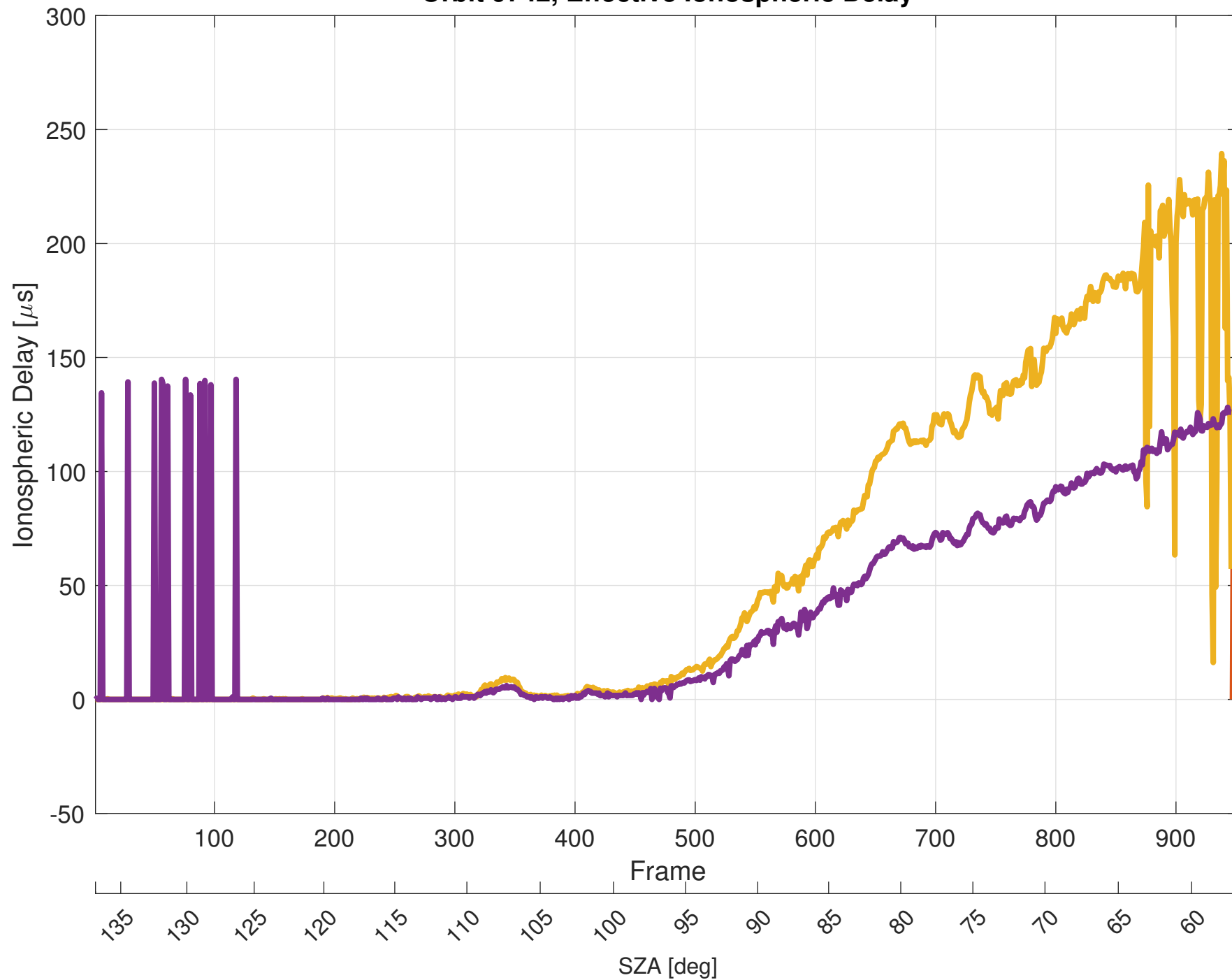
Orbit 9742, Effective Ionospheric Delay
