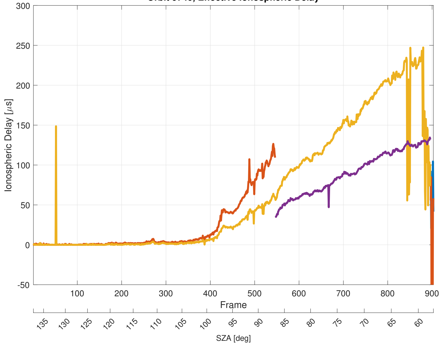
Orbit 9746, Effective Ionospheric Delay
