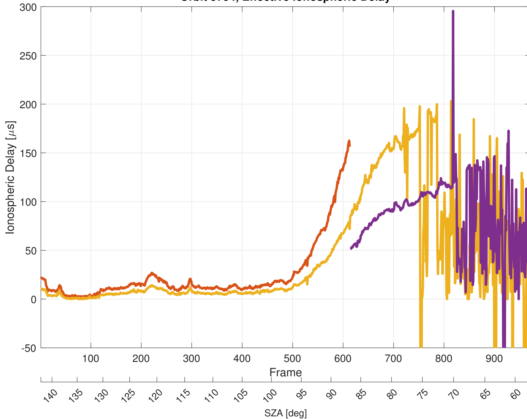
Orbit 9794, Effective Ionospheric Delay
